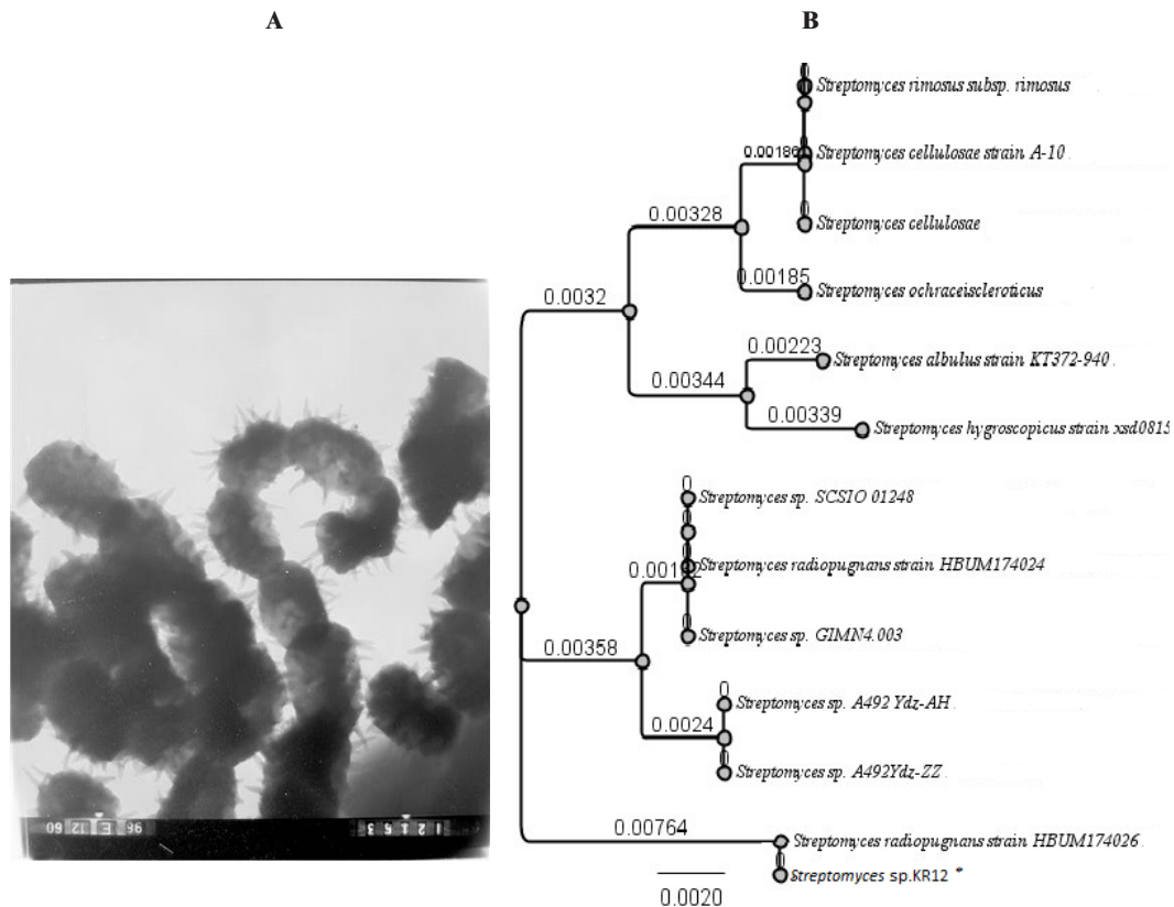
Fig. 1: A: Transmission electron microscope X 60 000 of KR12. B: Phylogenetic tree of 16S rRNA of Streptomyces radiopugnans KR12 and allied bacteria. The branching pattern was generated by the neighbor-joining method. Bar Jukes-Cantor distance of 0.002.
