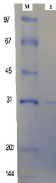
Fig 2: Molecular weight of keratinase isolated from Streptomyces radiopugnans KR12. by SDS-PAGE, M: protein standards employed were phosphorylase (97kDa), albumin (66kDa), ovalbumin (45kDa), carbonic anhydrase (30kDa), soybean trypsin inhibitor (20.1kDa), and \alpha -lactalbumin (14.4kDa), lane 2: Purified keratinase.
