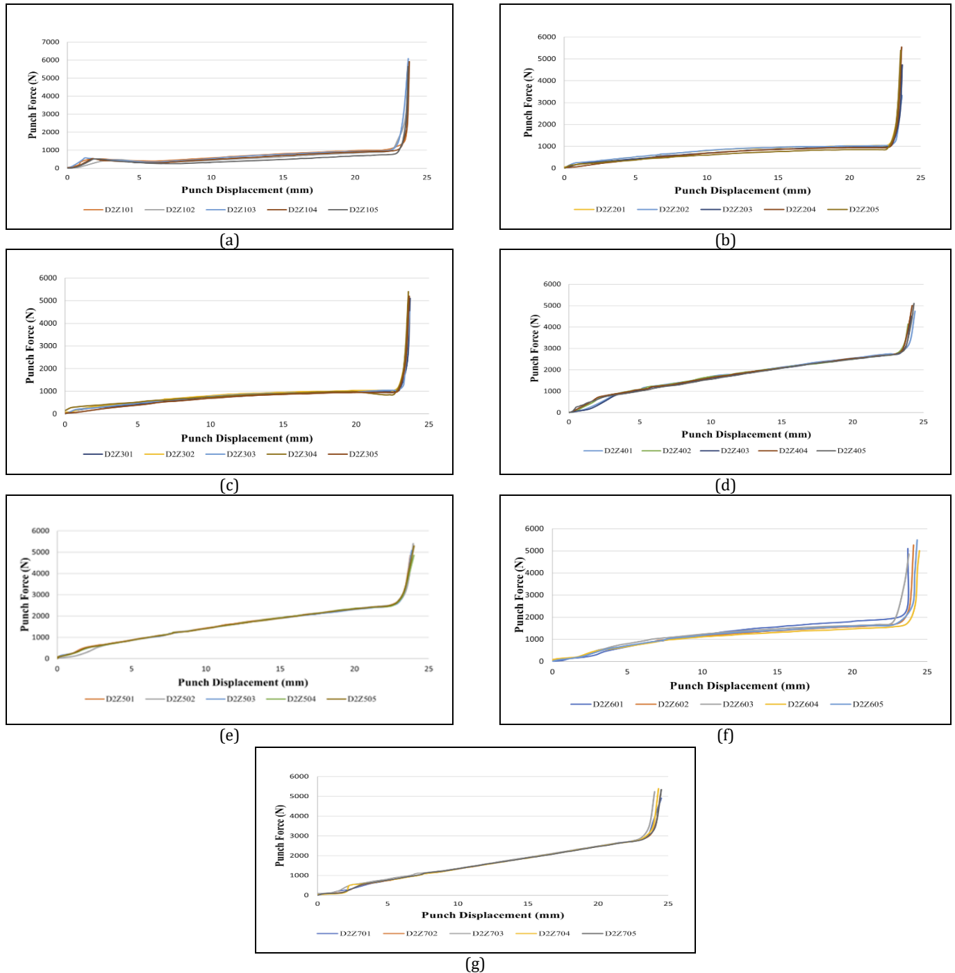
Figure 8. Punch force-displacement during deep drawing using various punch geometries. (a): Z1. (b): Z2. (c): Z3. (d): Z4. (e): Z5. (f): Z6. (g): Z7 punch geometries.
