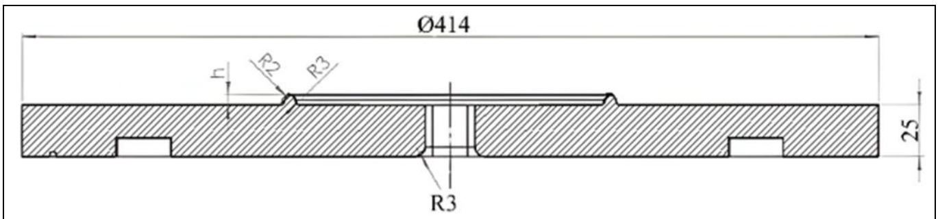
Figure 5. Geometry of the blank holder.
