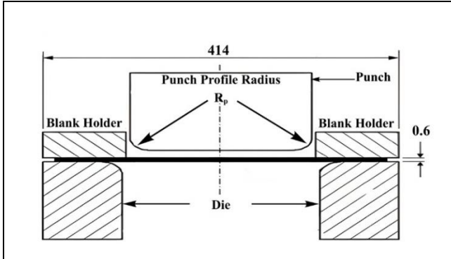
Figure 4. Schematic representation of drawing tools.
