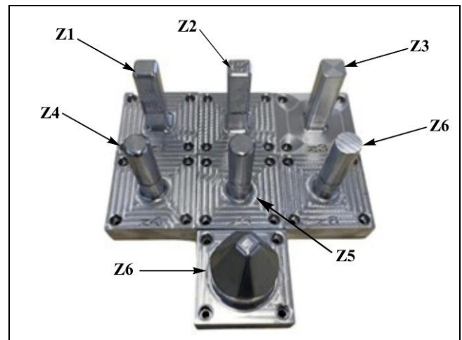
Figure 3. Seven different types of punch geometries.
