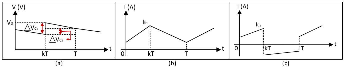
Figure 7. Waveforms. (a): Output voltage. (b): Input current. (c): Current through the C_1 capacitor.
