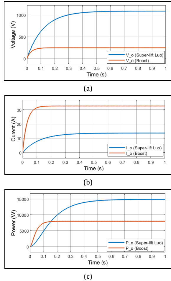
Figure 14. Output graphics. (a): voltage. (b): current. (c): power.
