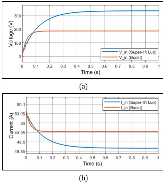
Figure 13. Input graphics. (a): Voltage. (b): Current.
