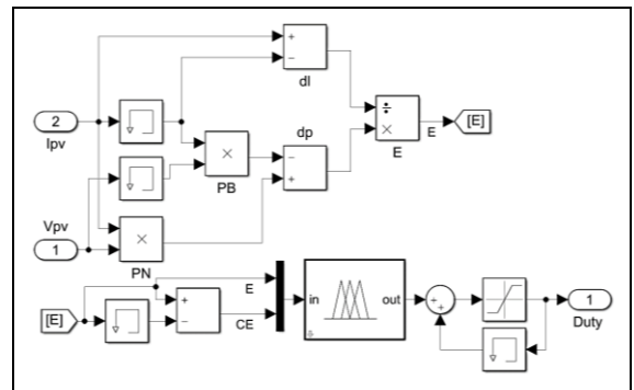
Figure 10. The internal structure of the developed FLC.
