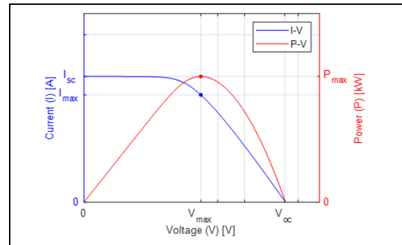
Figure 3. Current-voltage and power-voltage characteristics of a typical PV panel.
