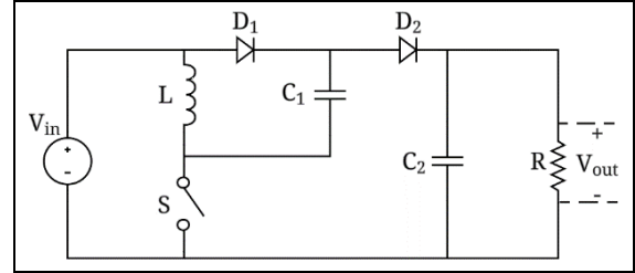
Figure 5. Circuit diagram of super-lift Luo converter.
