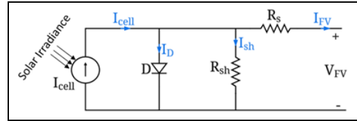
Figure 2. The single diode model of PV cell.
