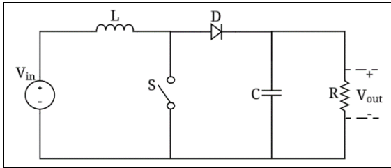
Figure 4. Circuit diagram of boost converter.
