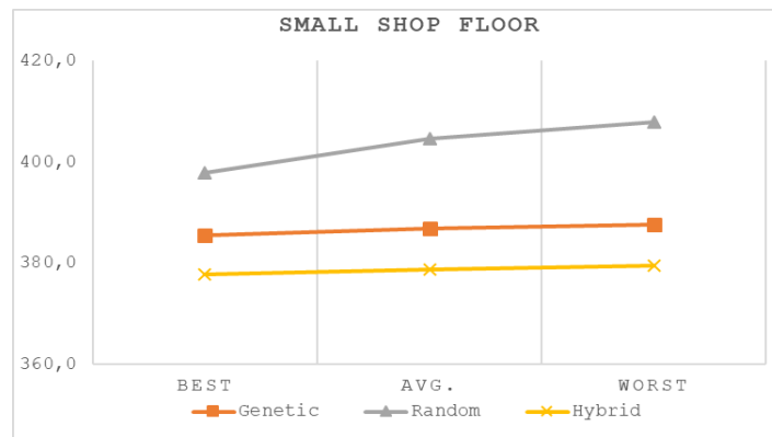
Figure 2. Small shop floor results
