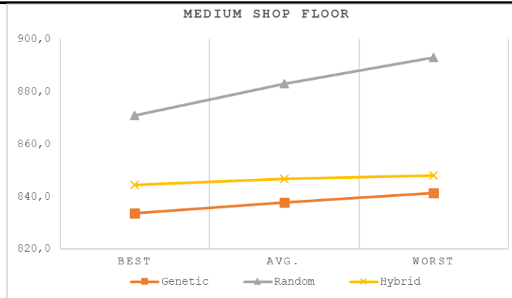
Figure 3. Medium shop floor results
