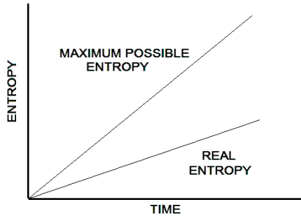
Fig. 2. Diagramm Time-Entropy.
