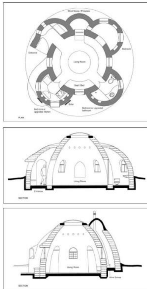
Figure 15: A simple plan of one of the houses built by cloud clay (Saeed Sun, 2012).
