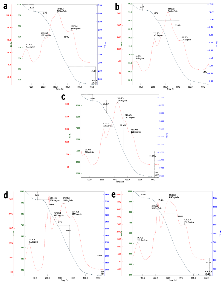
FIGURE 1. dTGA thermograms of; a) Salix babylonica , b) S. caprea , c) S. fragilis , d) Fraxinus excelsior and e) Betula pendula . In the figures, it is clearly shown that maximum degradations temperatures are visible in every steps.
