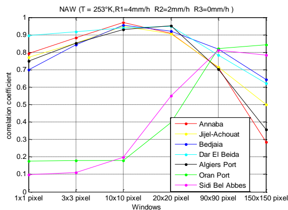
Figure 10. Correlation coefficient of different study area, day-by-day comparison, using different windows
