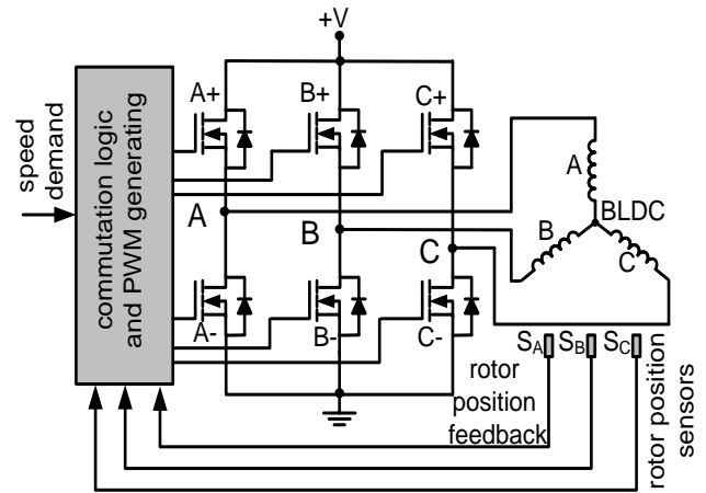
Figure 1. BLDC motor driving scheme.
