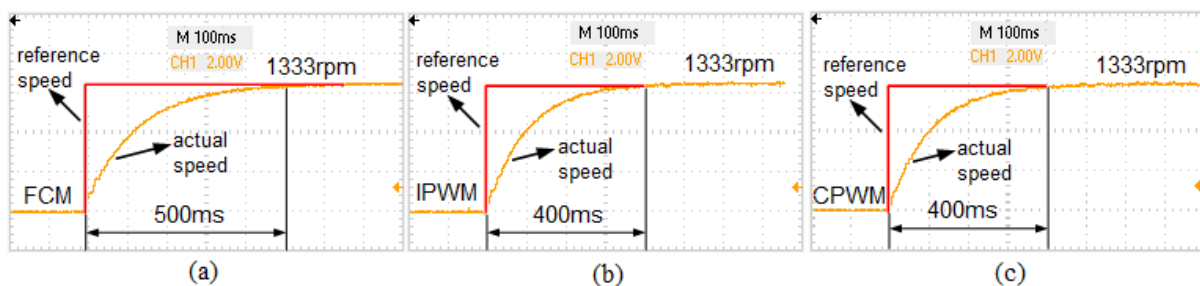
Figure 9. Speed up response of BLDC motor for three PWM current control methods for same speed under same load.
