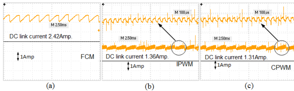
Figure 10. When BLDC motor working rated phase current (2.1 Amp.) DC link currents with respect to three PWM schemes.
