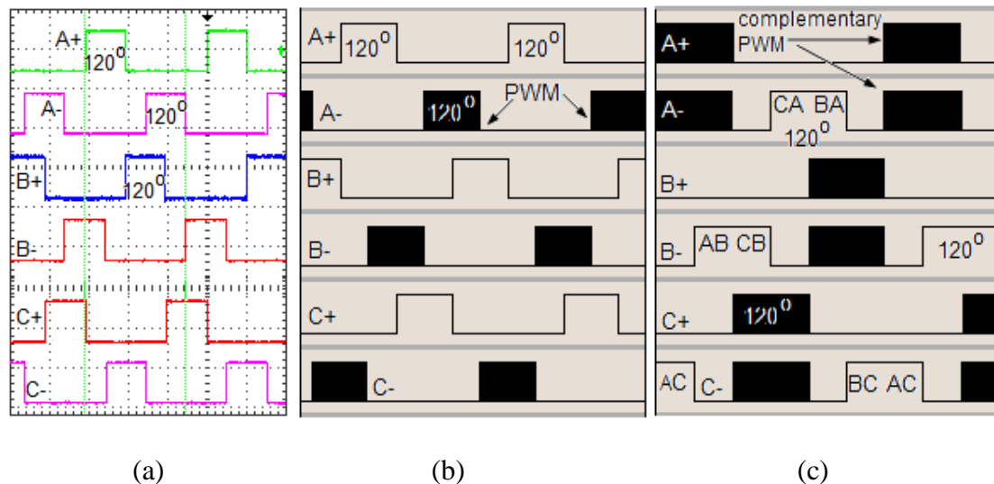
Figure 6. Inverter switching gate signals; (a) variable DC bus voltage, (b) independent PWM, (c) complementary PWM.
