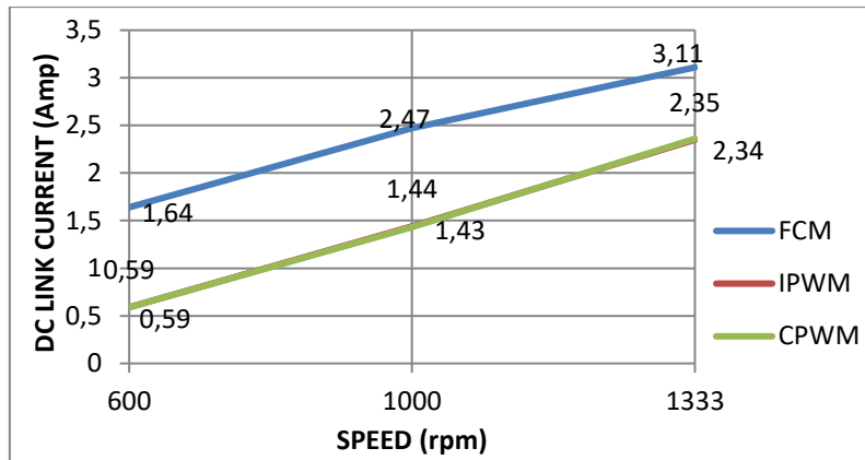
Figure 7. Inverter DC link currents when the DC generator load is 2\Omega .
