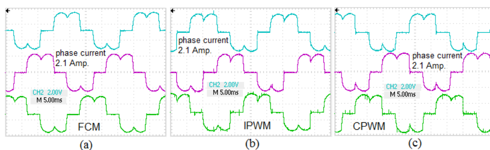
Figure 11. BLDC motor phase currents with respect to three PWM modes when the motor is working its rated phase current.
