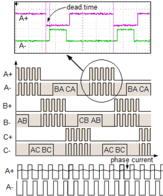
Figure 4. Complementary PWM switching method.
