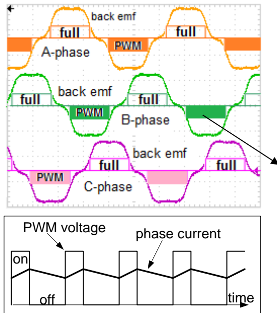
Figure 3. Structure of independent PWM switching mode.
