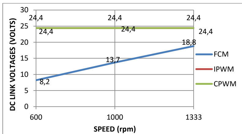
Figure 8. Inverter DC link Voltages when the DC generator load is 2.6\Omega .
