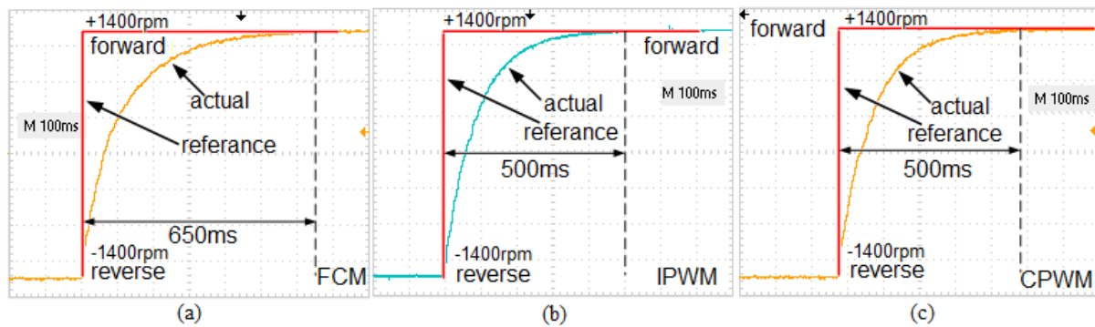
Figure 12. Reversible speed performance of BLDC motor according to three PWM schemes.
