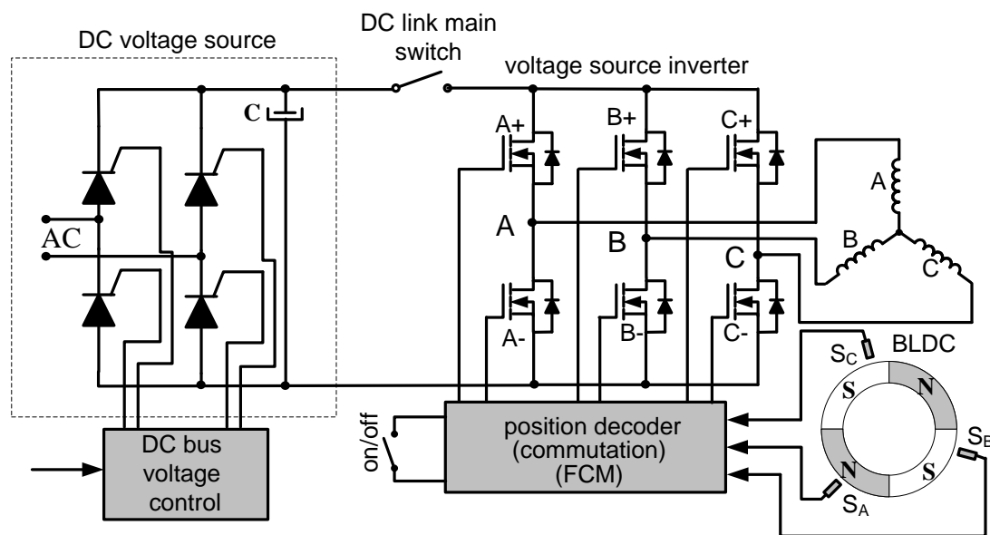
Figure 2. Variable DC Bus voltage BLDC motor driver.
