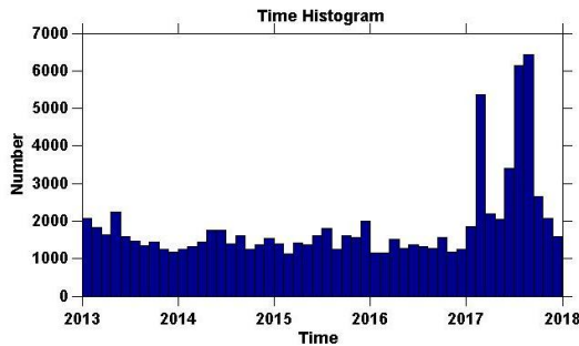
Figure 4. Earthquake-time histogram.
