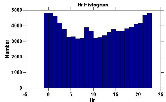
Figure 5. Earthquake-hour histogram.
