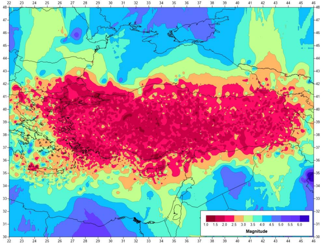
Figure11. Magnitude threshold map for Turkey and surrounding area computed by using the earthquakes in the time period 2013-2017.
