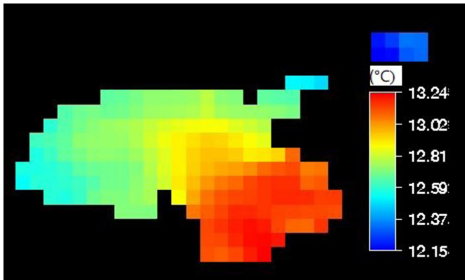
Figure 10. General average of SST of 210 images.
