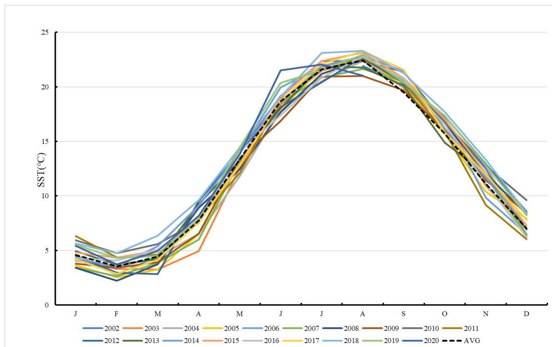
Figure 6. Monthly distribution of SST October, November 2002 and May, June 2003 are off the average.
