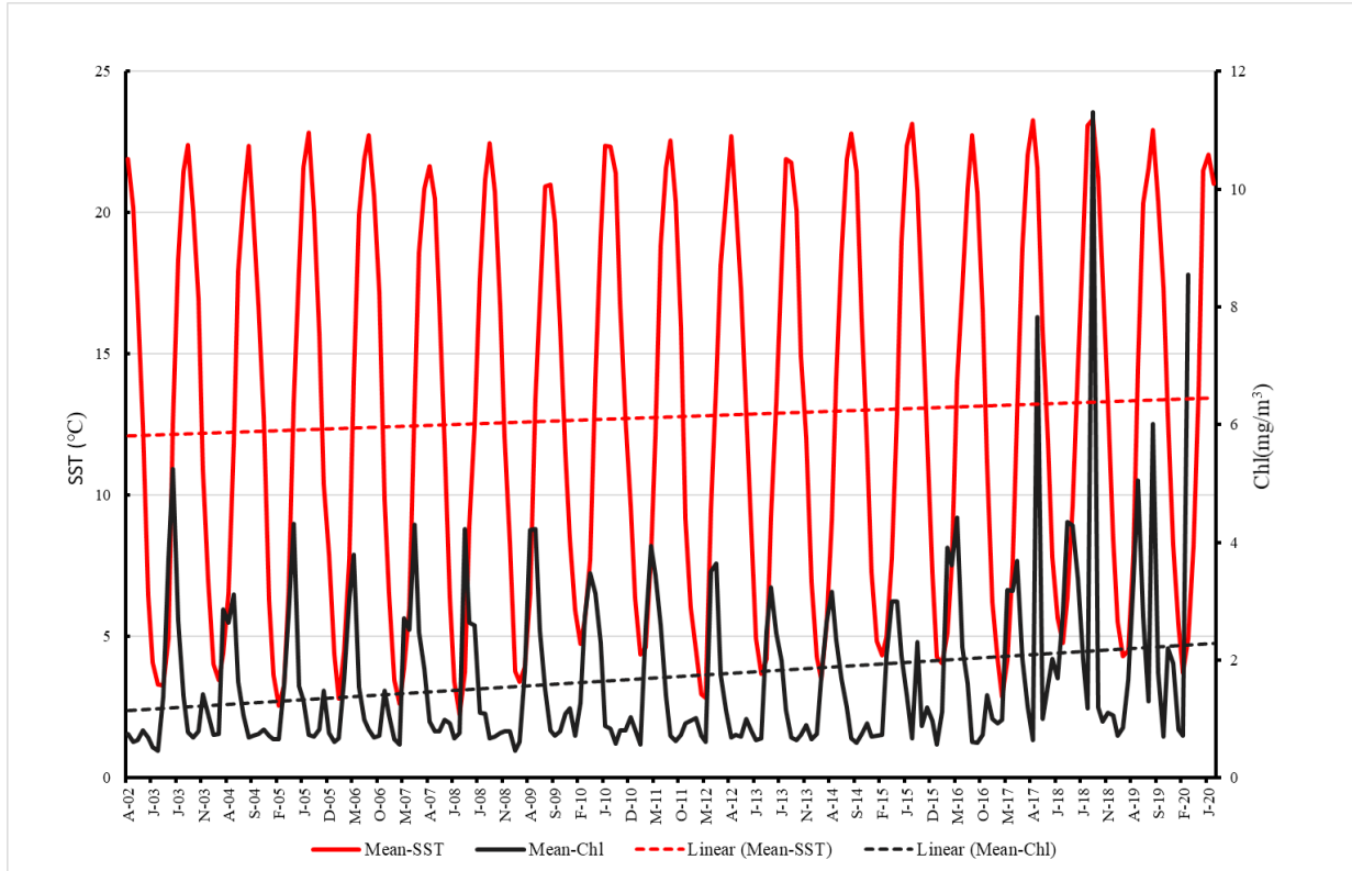
Figure 3. SST ( and Clorophyll (mg/m 3 ) variation of Lake Van from August 2002 to April 2020.
