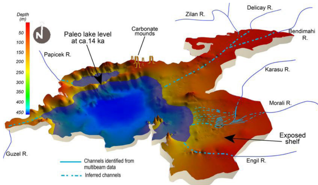
Figure 1. Bathymetry of Lake Van (Cukur et al., 2015).
