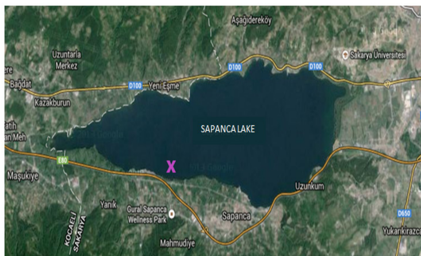
Figure 1. The location of the sampling site (X) on the map of the study area, Sapanca Lake, Turkey.
