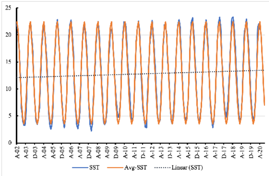
Figure 9. Long-term SST distribution with average and trendline
