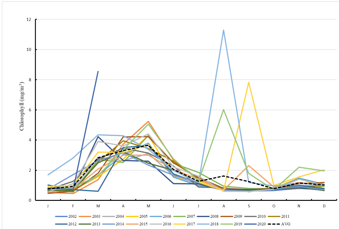
Figure 5. Monthly distribution of chlorophyll-a pigment concentration of lake Van
