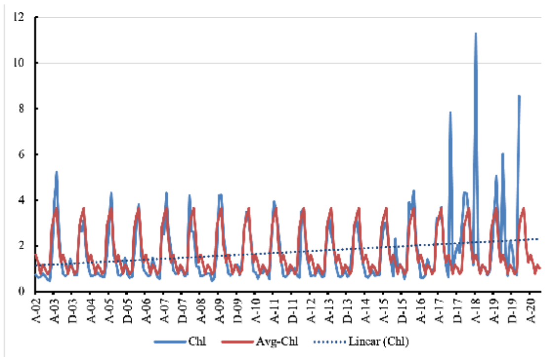
Figure 8. Long term chlorophyll-a pigment concentration along with the average variation of the Lake Van from August 2002 to April 2020.
