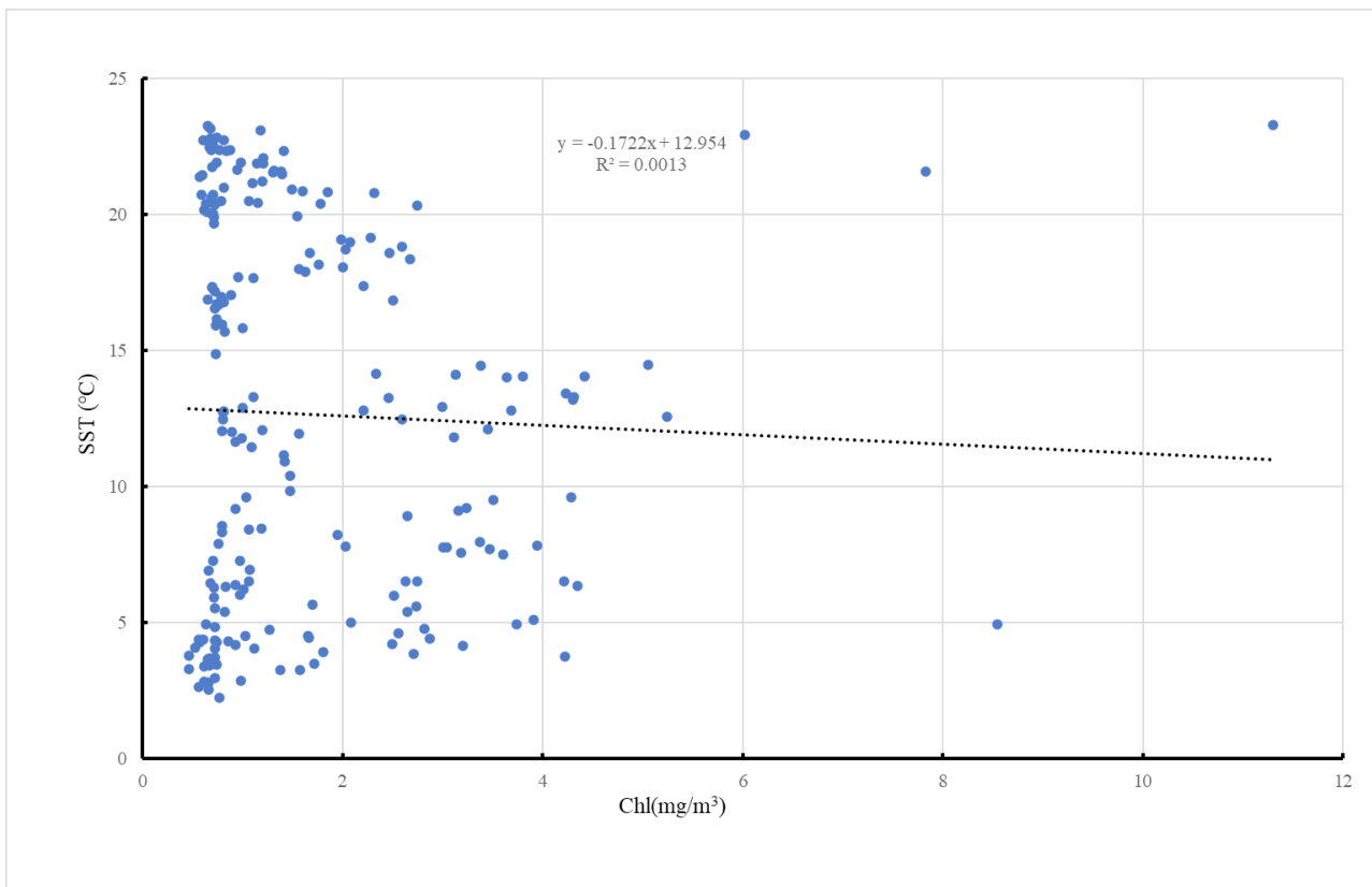
Figure 4. Relationship between SST and Chl-a values from August 2002 to April 2020.
