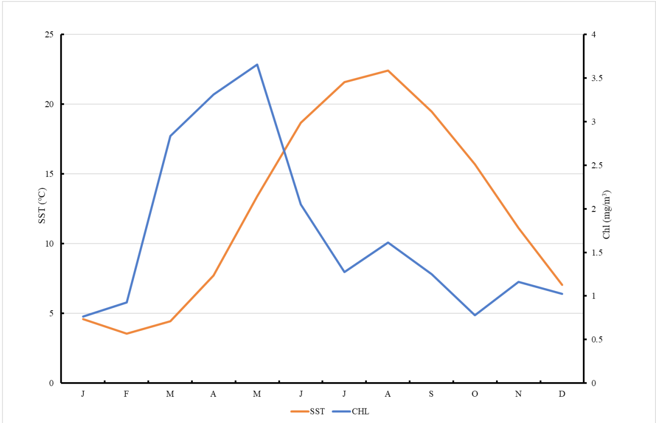
Figure 7. Monthly distribution SST and Chl-a average of Lake Van
