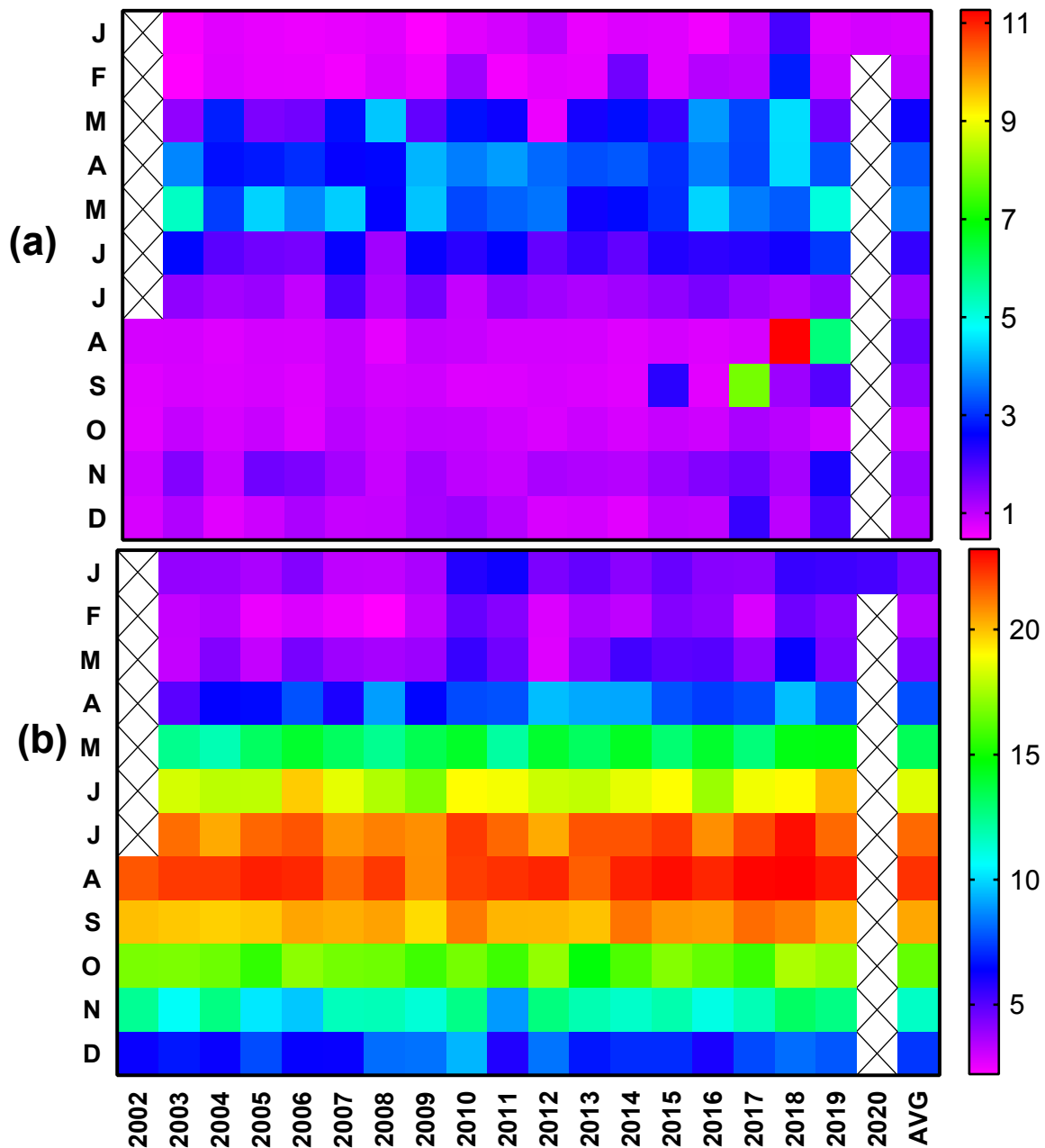
Figure 11. Monthly heatmap of Chlorophyll-a pigment concentration ( \text{mg}/\text{m}^3 ) (a) and SST ( ^{\circ}\text{C} ) (b).
