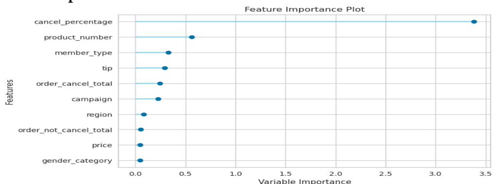
Figure 6. Feature Importance Plot for Logistic Regression
