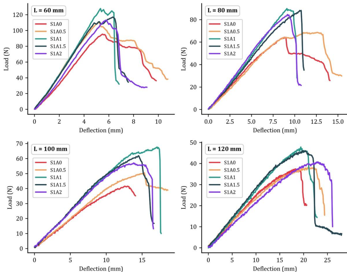
Figure 3. Load-deflection curves of the composite sample groups under three-point bending.
