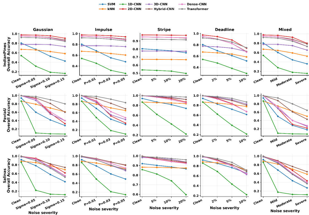
Figure 4. Overall accuracy across noise levels.
