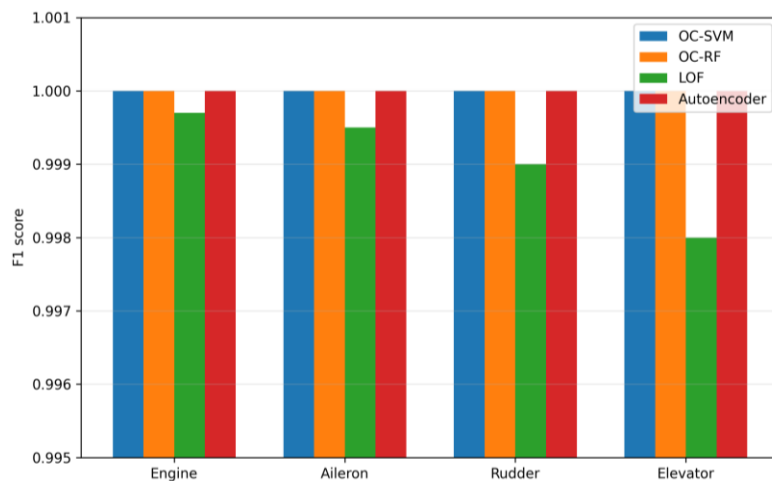
Figure 10. F1-score comparison of four methods by fault type.
