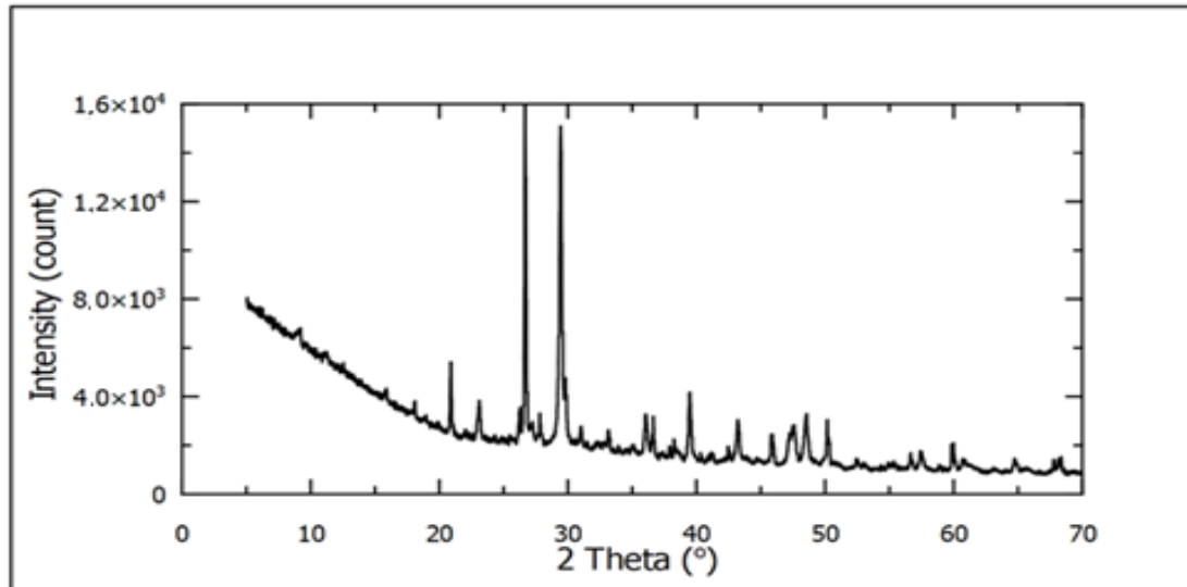
Figure 2. XRD diffractogram of concrete debris.
