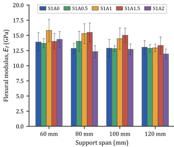
Figure 5. Flexural modulus by support span.
