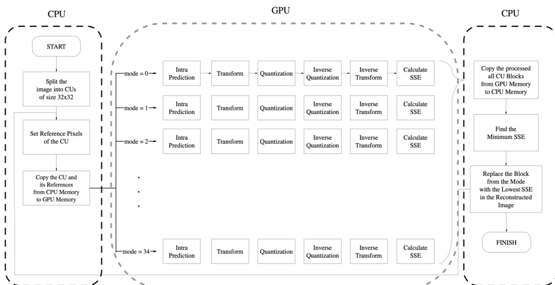
Figure 3. General block diagram of parallel calculation of intra prediction model.
