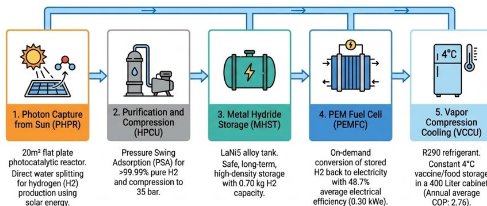
Figure 1. Schematic diagram of the integrated photocatalytic H 2 -PEM fuel cell-off-grid cold storage system with subsystem boundaries.
