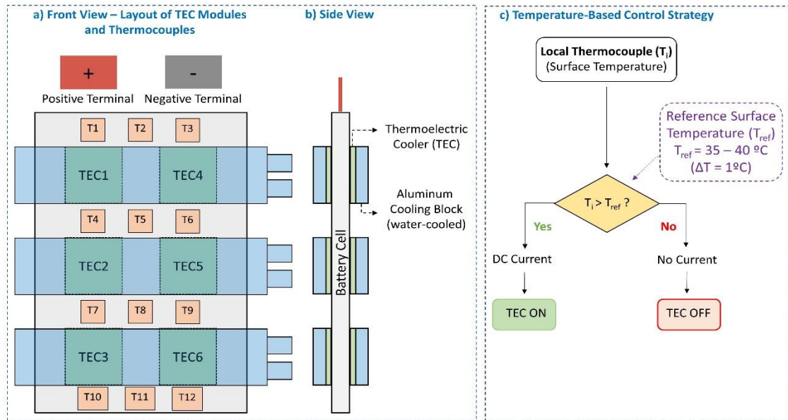
Figure 1. Schematic illustration of the thermoelectric battery thermal management system and temperature-based control strategy.
