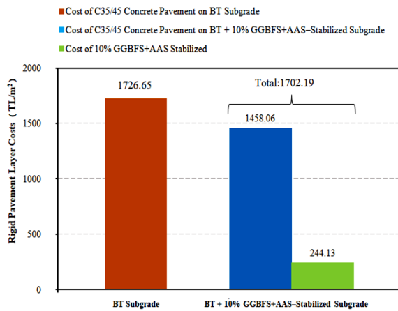
Figure 9. Concrete pavement and subgrade stabilization costs for untreated and 10% GGBFS+AAS-stabilized BT.
