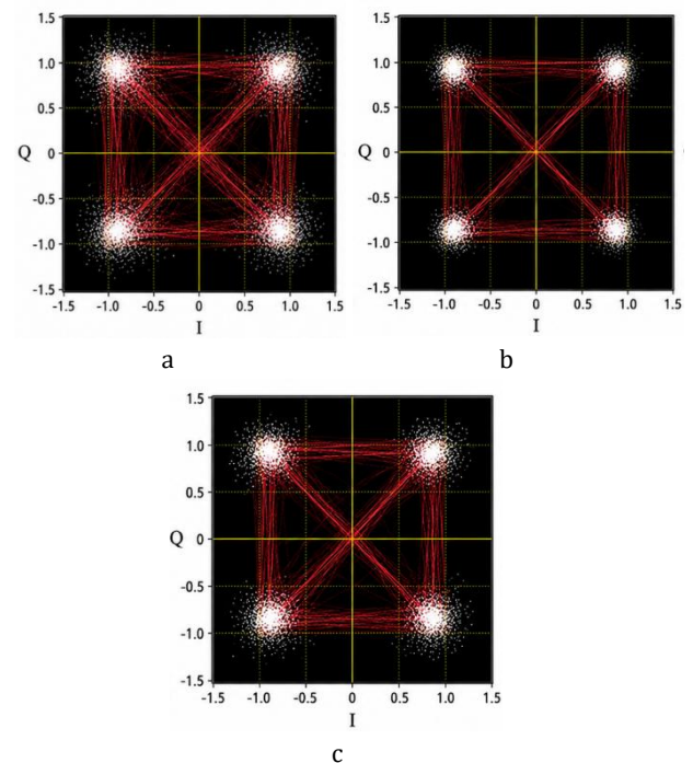
Figure 8. Representative link-level QPSK constellation diagrams obtained using the 2 \times 2 OTA software-defined-radio testbed: (a) 5.18 GHz, (b) 5.50 GHz, and (c) 5.825 GHz.
