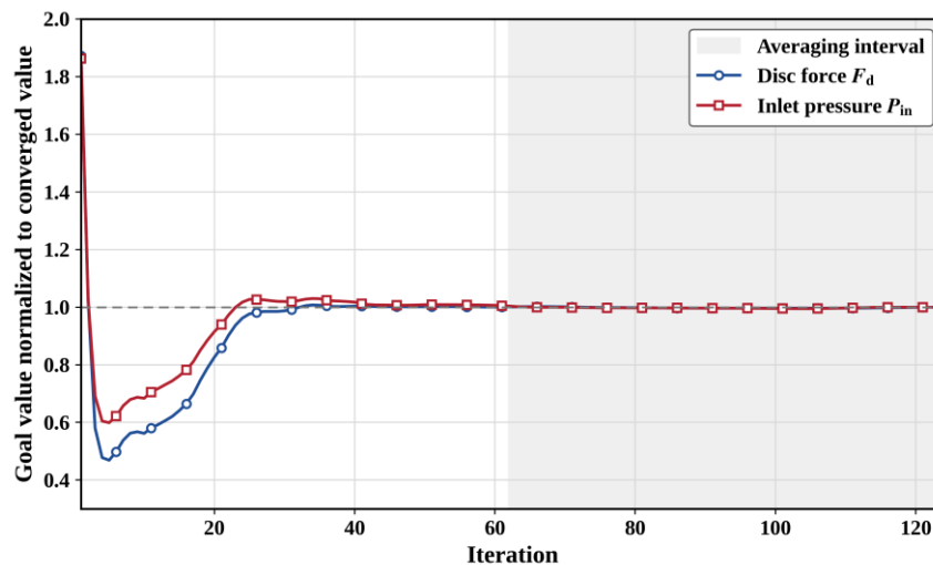
Figure 4. Iterative convergence of the monitored goals for the conventional design at the most throttled position (30 degrees). The hydrodynamic disc force and the inlet static pressure, each normalized to its converged value, settle onto a stable plateau, and the shaded band marks the averaging interval over which the goals are evaluated.
