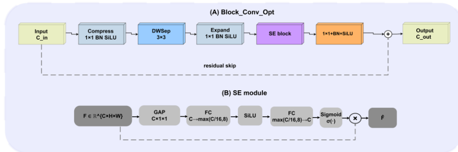
Figure 2. Block_Conv_Opt internal structure (A) and squeeze-and-excitation recalibration module (B). (A) Input features are first compressed to \text{mid} = \max(\text{C}_{\text{out}}/2, 16) channels via 1x1 convolution, processed by a depth-wise separable convolution ( \text{mid} \rightarrow \text{mid} ), expanded back to \text{C}_{\text{out}} , and recalibrated by SE before the residual addition; a final 1x1+BN+SiLU layer produces the block output. The residual skip applies a 1x1 projection when \text{C}_{\text{in}} \neq \text{C}_{\text{out}} . (B) The SE module performs global average pooling, followed by two fully connected layers with bottleneck width m = \max(C/16, 8) , and sigmoid gating applied channel-wise.
