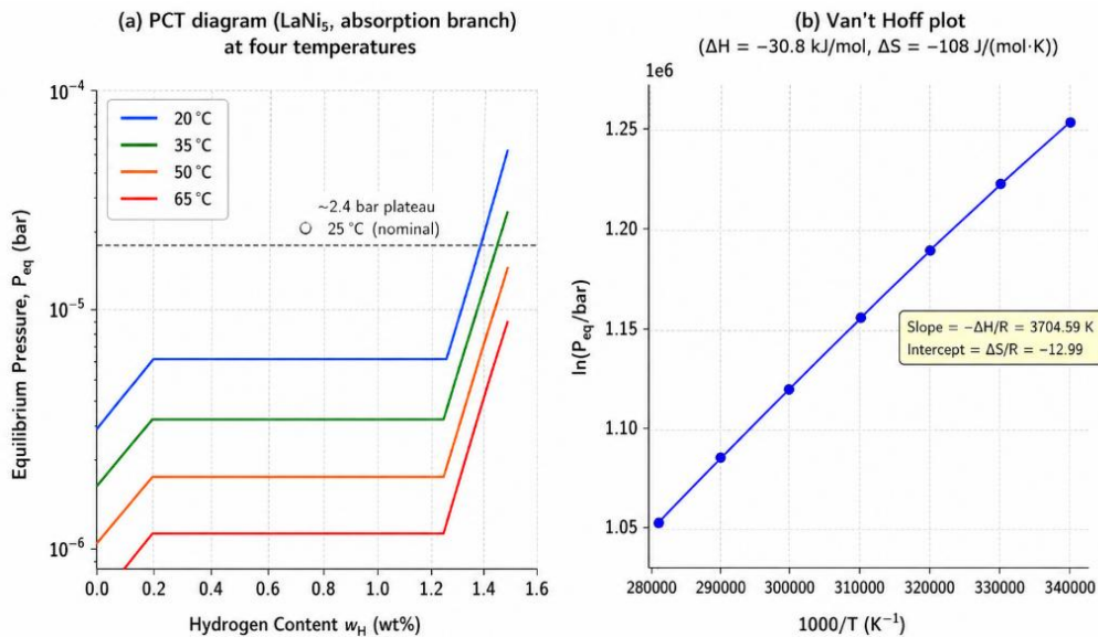
Figure 3. LaNi 5 metal hydride characteristics: (a) PCT diagram (absorption branch) at four temperatures; (b) van't Hoff plot with \Delta H and \Delta S annotations.
