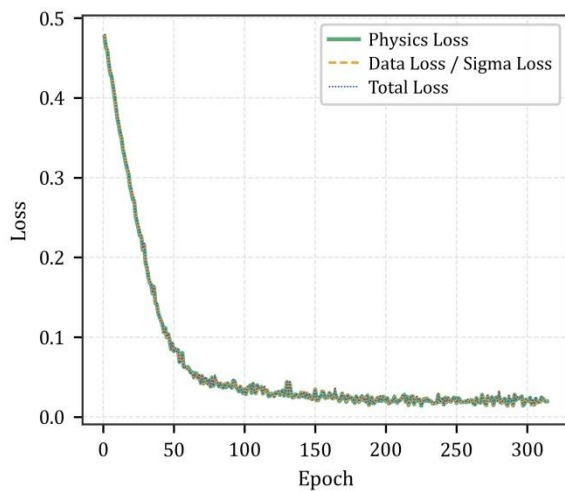
Figure 7. Loss-epoch graph of the PINN model.
