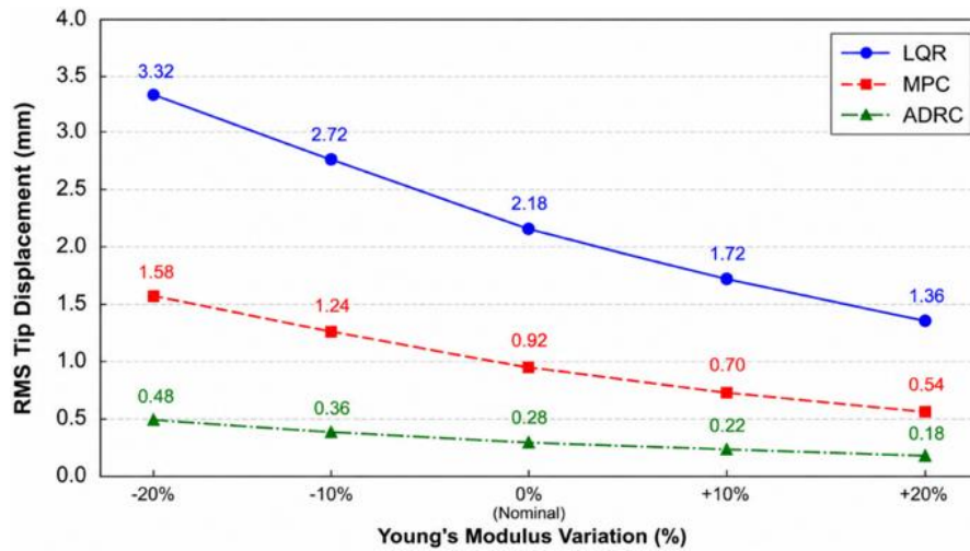
Figure 12. Variation of RMS tip displacement with Young Modulus uncertainty
