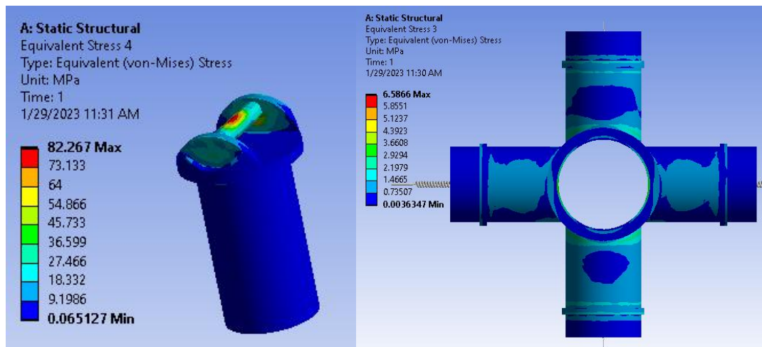
Figure 4. The generated mesh for the structural analysis and the stress values on compressor components.
