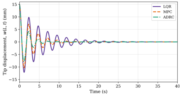
Figure 9. Tip displacement responses under Scenario 3.
