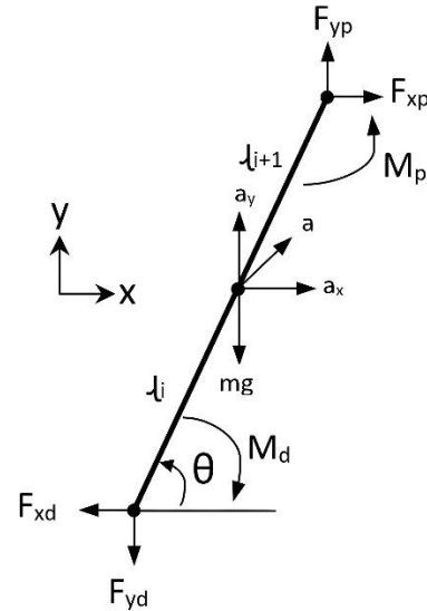
Figure 3. Free-body diagram illustrating the net forces, moments, and accelerations of a single segment.
