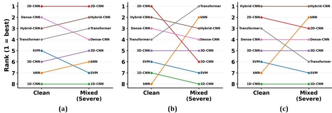
Figure 5. Model ranking shift from clean to mixed noise: (a) Indian Pines, (b) Pavia University, (c) Salinas.
