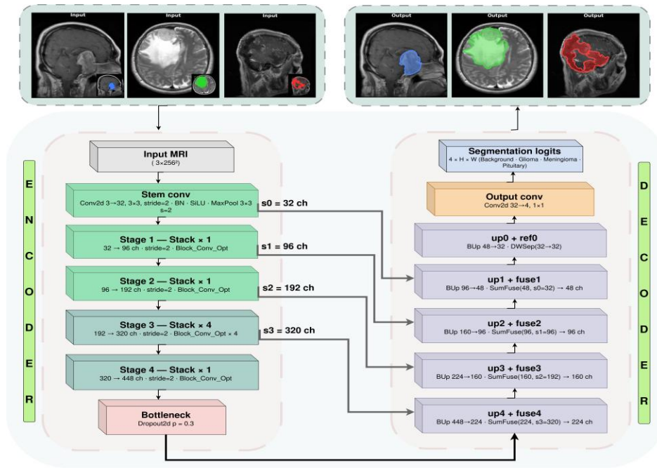
Figure 1. A3Net encoder-decoder overview. Channel widths at each stage are indicated above the blocks; skip connections s0–s3 are shown as lateral arrows. \oplus denotes element-wise summation in SumFuse modules. The final ref0 stage applies a single DWSep without a skip connection; the output 1x1 convolution produces a 4-class prediction map ( 4 \times 256^2 ).
