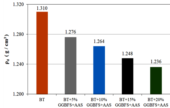
Figure 5. Maximum dry unit weight results of the Standard Proctor test.
