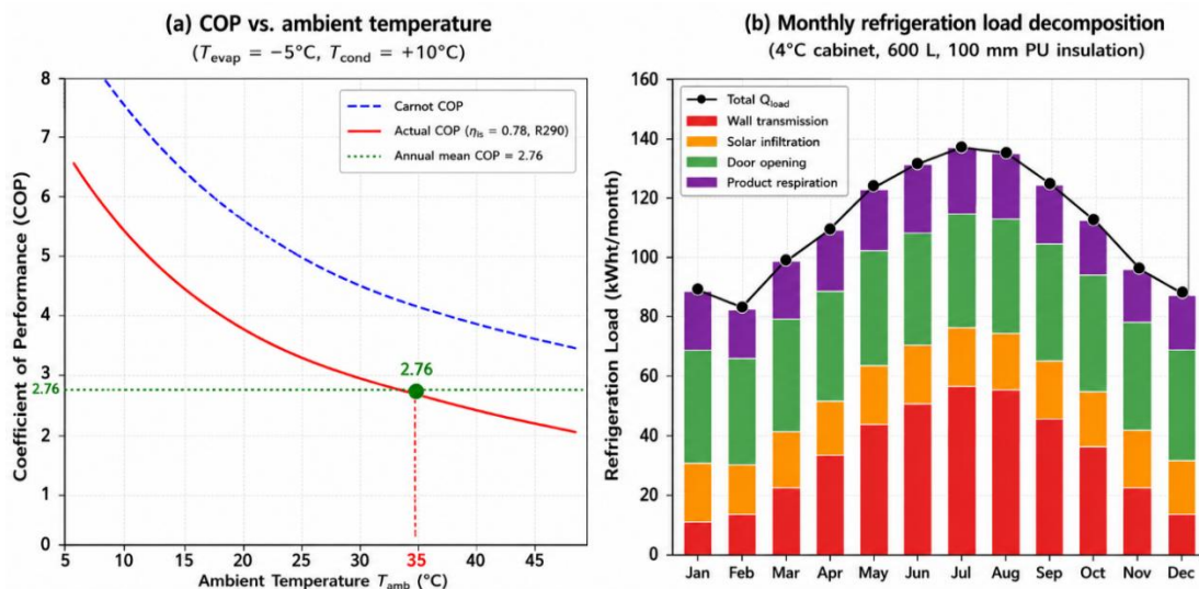
Figure 5. Vapor-compression refrigeration cycle (R290) performance: (a) COP vs. ambient temperature with Carnot COP reference; (b) monthly refrigeration load decomposition by component.
