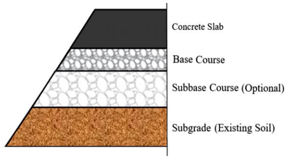
Figure 4. Cross-section of the rigid pavement (Kök, 2019; Geçkil et al., 2024).
