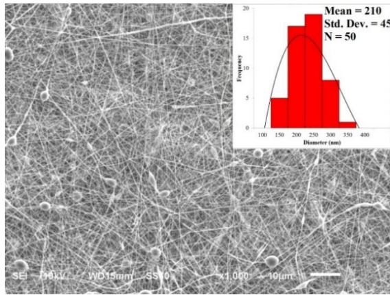
(a) Sample 5 (10.0 wt% concentration, 1.2 mL/h flow rate, 22G needle diameter) Thinnest fiber: 210 ± 45 nm
