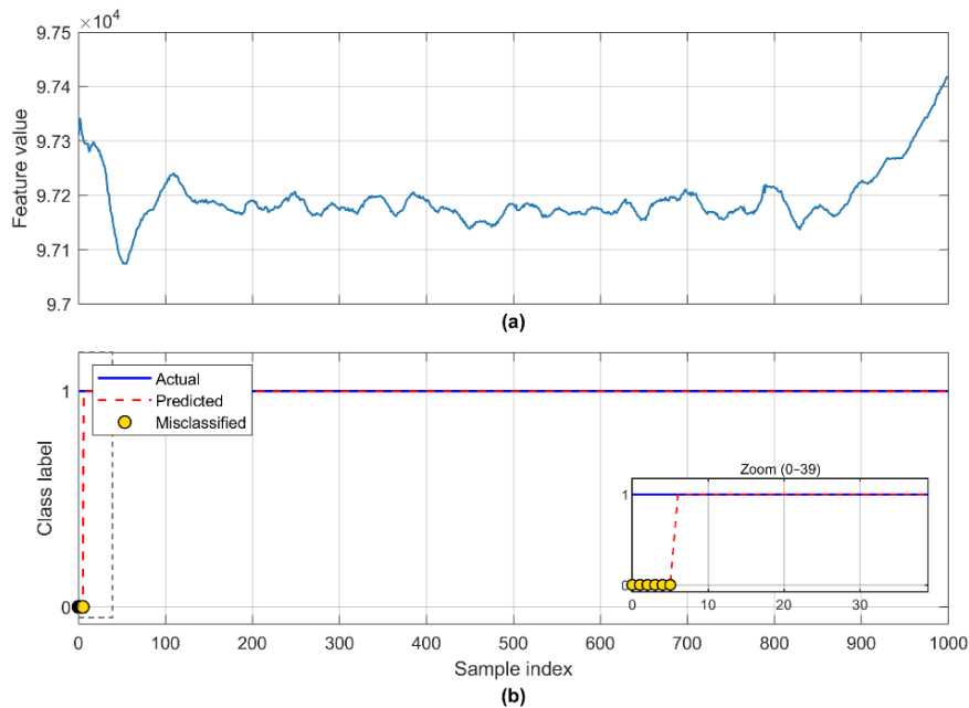
Figure 9. LOF results for engine fault on a representative sample window. (a) resampled feature, (b) actual and predicted class labels.
