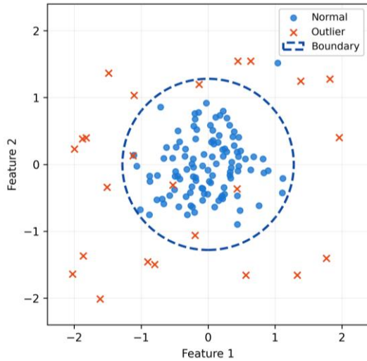
Figure 4. Schematic representation of one-class support vector machine (OC-SVM) (Muñoz and Moguerza, 2004).
