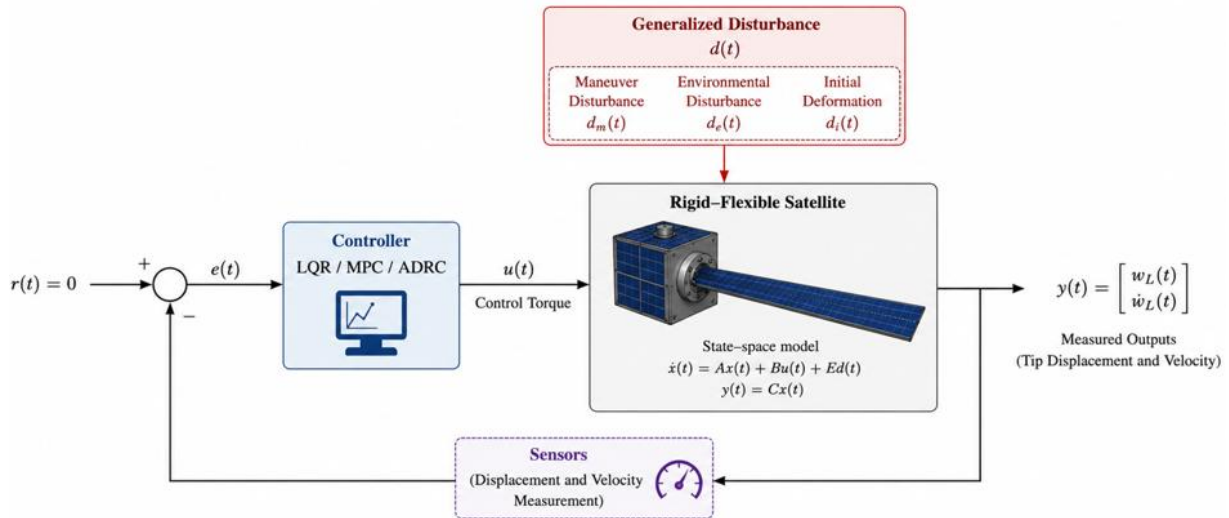
Figure 2. Feedback control architecture of the rigid-flexible satellite system
