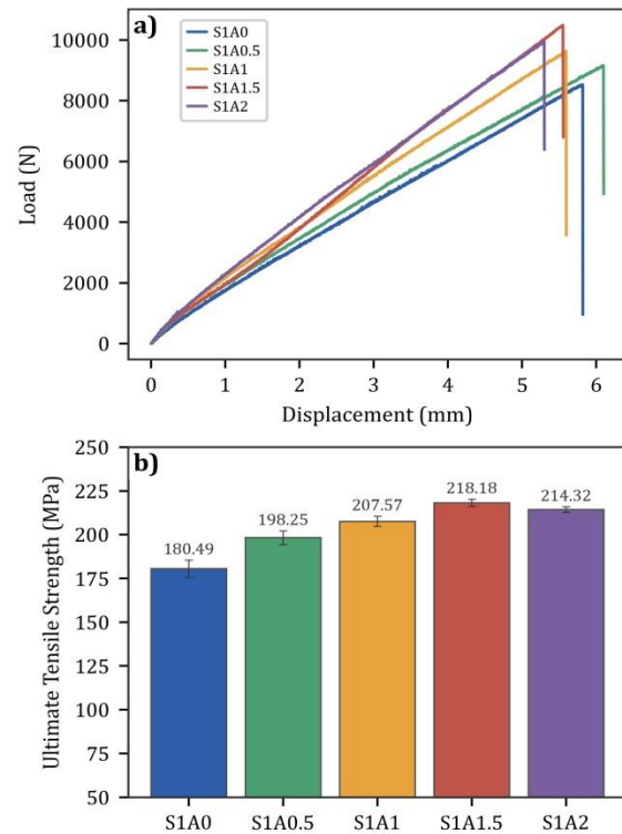
Figure 6. (a) Load–displacement curves and (b) ultimate tensile strength of the composite sample groups.
