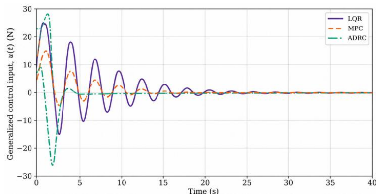
Figure 3. Tip displacement responses under Scenario 1.
