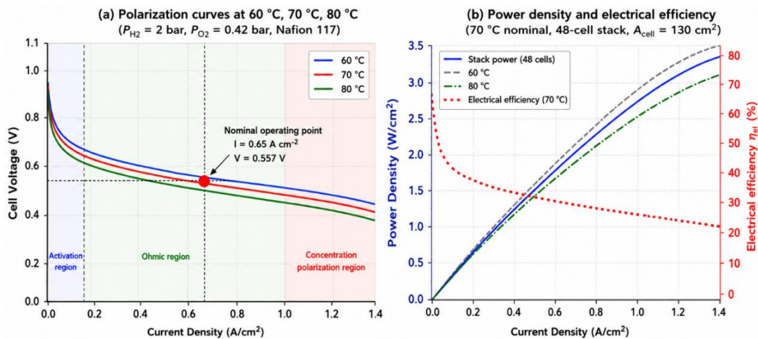
Figure 4. PEM fuel cell electrochemical performance: (a) polarization curves at 60°C, 70°C, and 80°C; (b) power density and electrical efficiency at 70°C.
