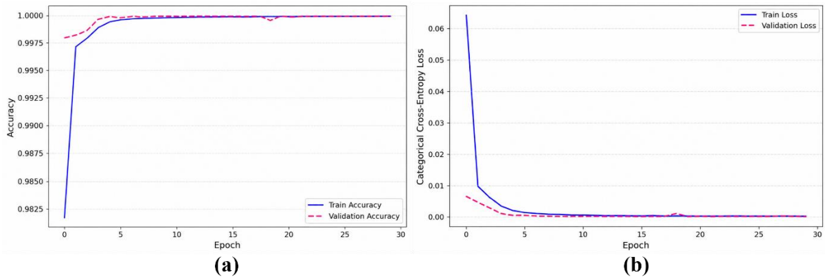
Figure 3. Accuracy and loss trends of the proposed DCNN model during training: (a) training and validation accuracy, and (b) training and validation loss.
