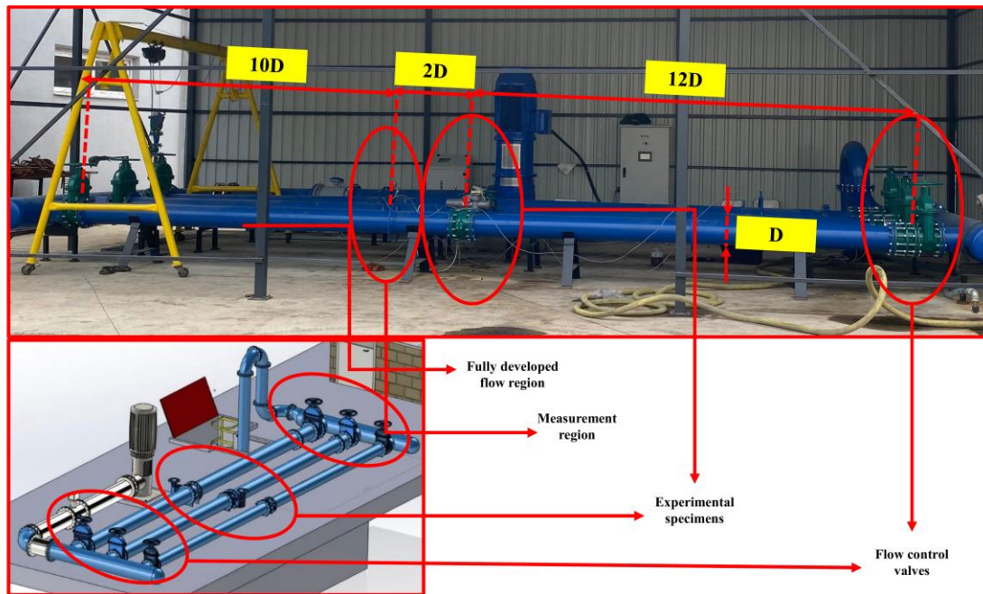
Figure 1. Experimental flow-bench layout of the DN350 line. According to TS EN 1267, the straight-pipe development lengths before and after the valve and the pressure measurement points were determined so that valve-induced disturbances would not reach the measurement sections (top, the physical setup; bottom, the CAD layout of the test circuit). D denotes the nominal diameter.
