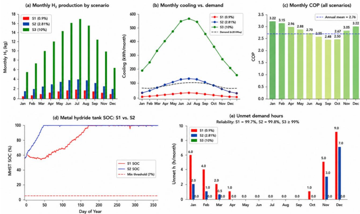
Figure 6. Annual dynamic simulation results ( A_r=20\text{m}^2 ): (a) monthly \text{H}_2 production by scenario; (b) monthly cooling output vs. demand; (c) monthly average COP; (d) metal hydride tank daily state of charge (SOC) (S1 vs. S2); (e) monthly unmet demand hours.
