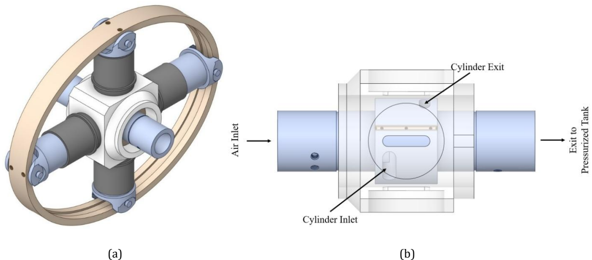
Figure 1. (a) Schematics of the designed compressor and (b) the inlet and exit ports
