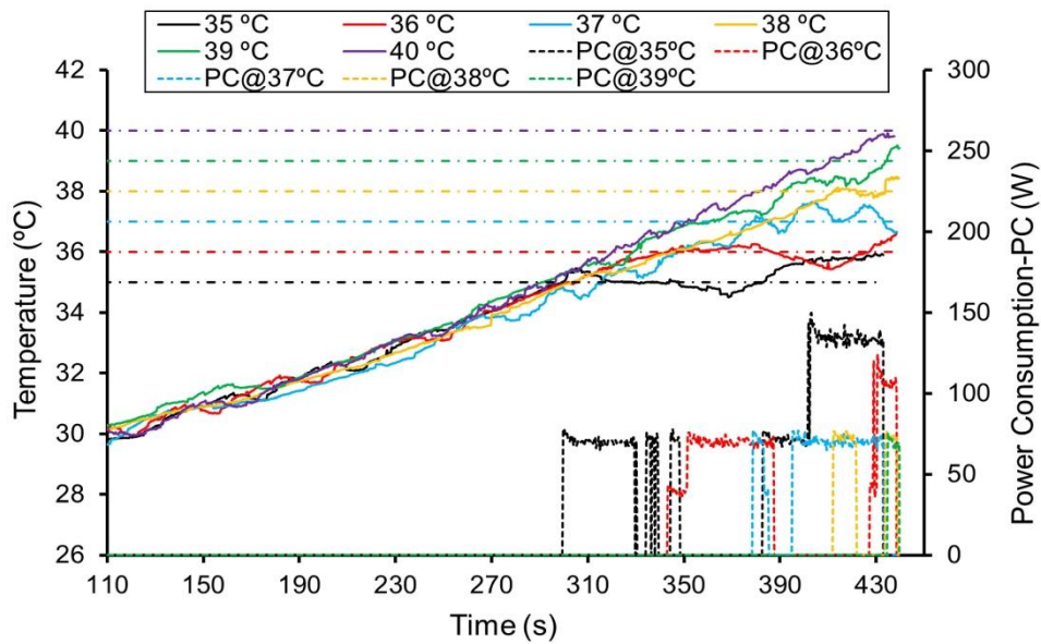
Figure 4. Battery surface temperature regulation and corresponding total TEC power consumption under different reference temperature settings.
