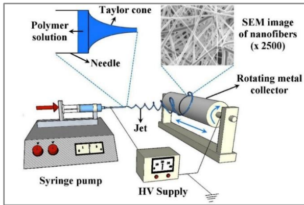
Figure 1. Schematic of an electrospinning setup (Aydemir et al., 2025).
