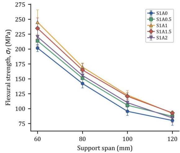
Figure 4. Span dependence of flexural strength.
