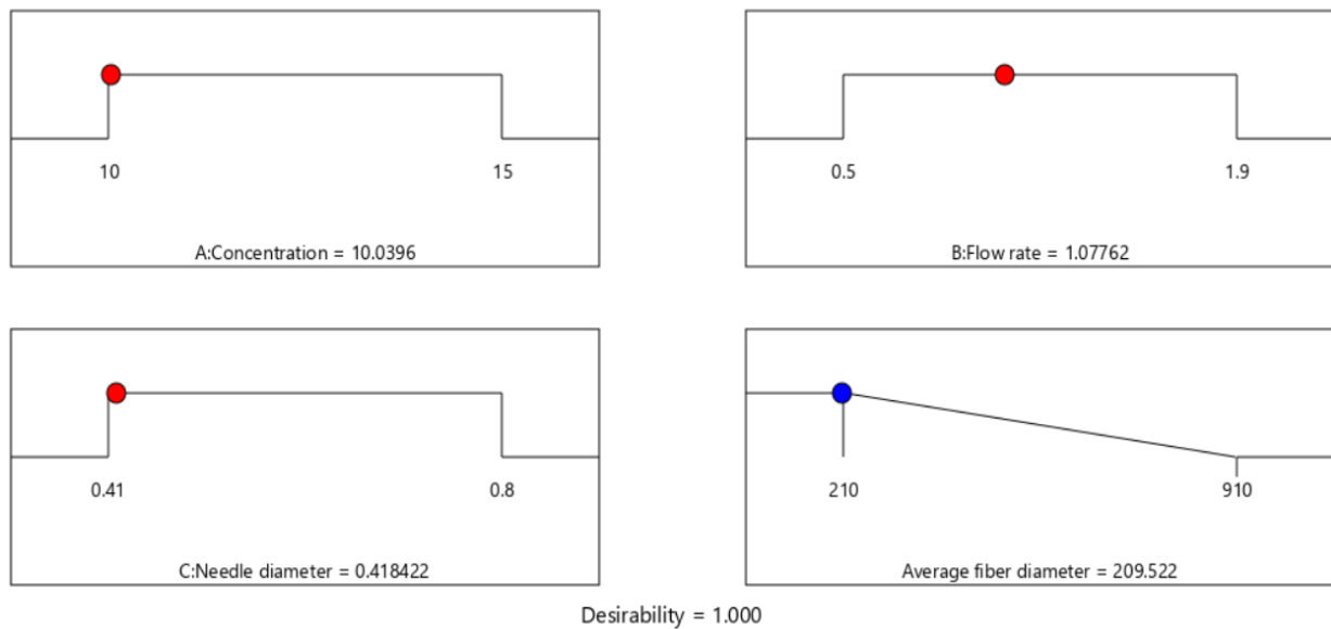
Figure 4. Desirability ramp plots for numerical optimization targeting minimum AFD in the r-PET electrospinning process.
