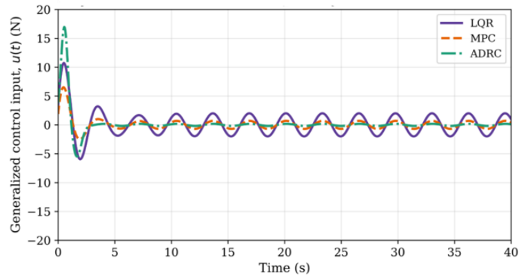
Figure 7. Generalized control input responses under Scenario 2.
