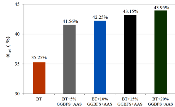
Figure 6. Optimum moisture content results of the Standard Proctor test.
