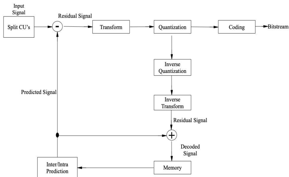
Figure 1. Basic Structure of the HEVC Intra Prediction Implementation.
