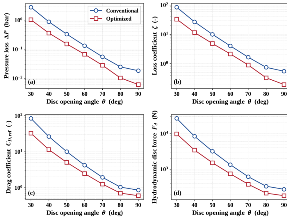
Figure 7. Hydraulic performance comparison of the conventional and optimized designs as a function of the opening angle (logarithmic scale): (a) valve pressure loss \Delta P , (b) dimensionless loss coefficient \zeta , (c) reference drag coefficient C_{D,ref} and (d) hydrodynamic force F_d on the disc. The optimized disc remains below the conventional disc at every angle. F_d is an indicator of the required actuation torque.
