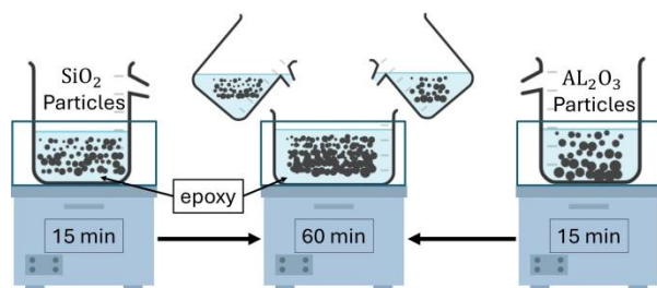
Figure 1. Mixing process of the particles and epoxy resin.
