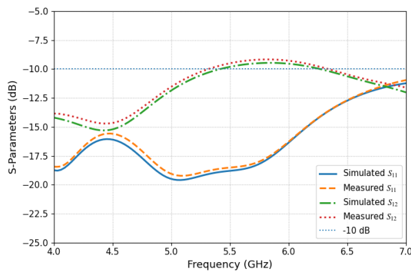
Figure 6. Simulated and measured S_{11} and S_{12} responses of the proposed symmetrical two-port MIMO antenna.
