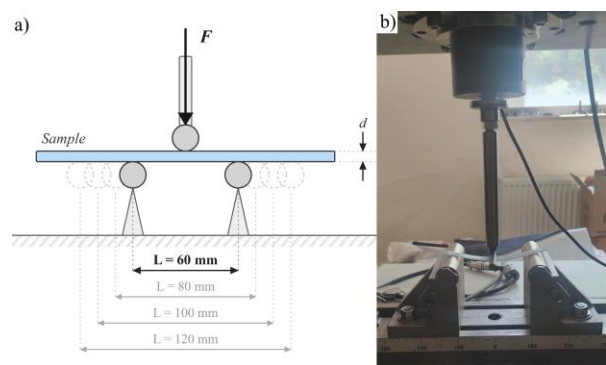
Figure 2. (a) Schematic of the three-point bending test setup; (b) photograph of the experimental setup.
