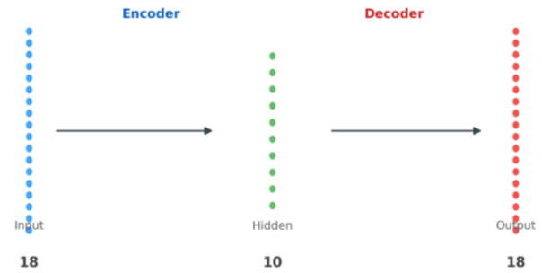
Figure 7. Autoencoder architecture used in this study (18–10–18 neurons) (Park et al., 2021).
