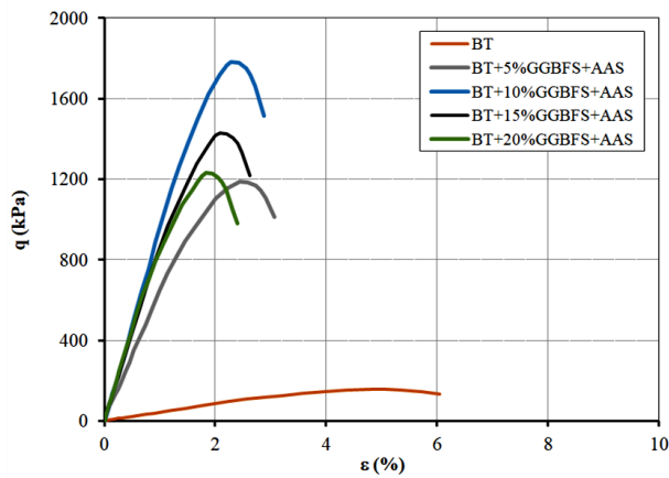
Figure 7. Stress-strain behavior of BT and GGBFS+AAS modified mixtures subjected to 28-day curing.
