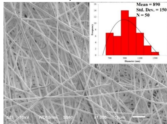
(d) Sample 8 (15.0 wt% concentration, 1.2 mL/h flow rate, 18G needle diameter) AFD of the sample with the widest needle diameter sharing the same concentration and flow rate as Sample 4 : 890 ± 150 nm
