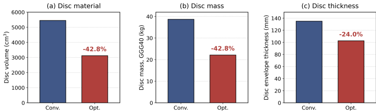
Figure 3. Geometric comparison of the conventional and optimized discs derived from the STEP models: (a) disc material volume, (b) disc mass for GGG40 spheroidal graphite cast iron, (c) disc envelope thickness. The optimized disc redistributes and removes material to obtain a thinner, flow-aligned lens-type profile.
