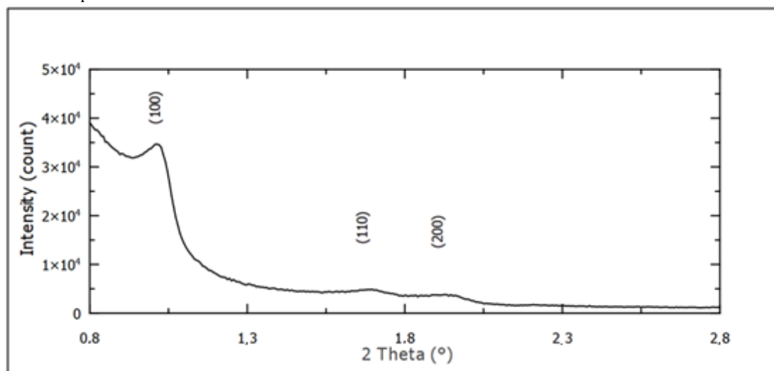
Figure 4. XRD diffractogram of synthesized SBA-15.
