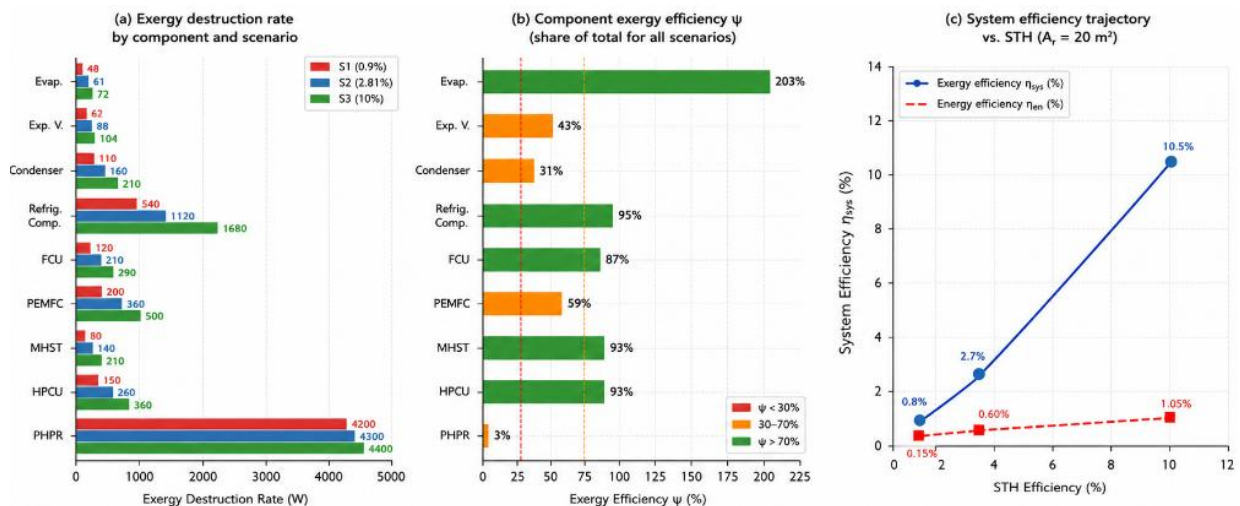
Figure 8. Exergy analysis: (a) exergy destruction rate by component and scenario; (b) component exergy efficiency \psi ; (c) system efficiency trajectory vs. STH.
