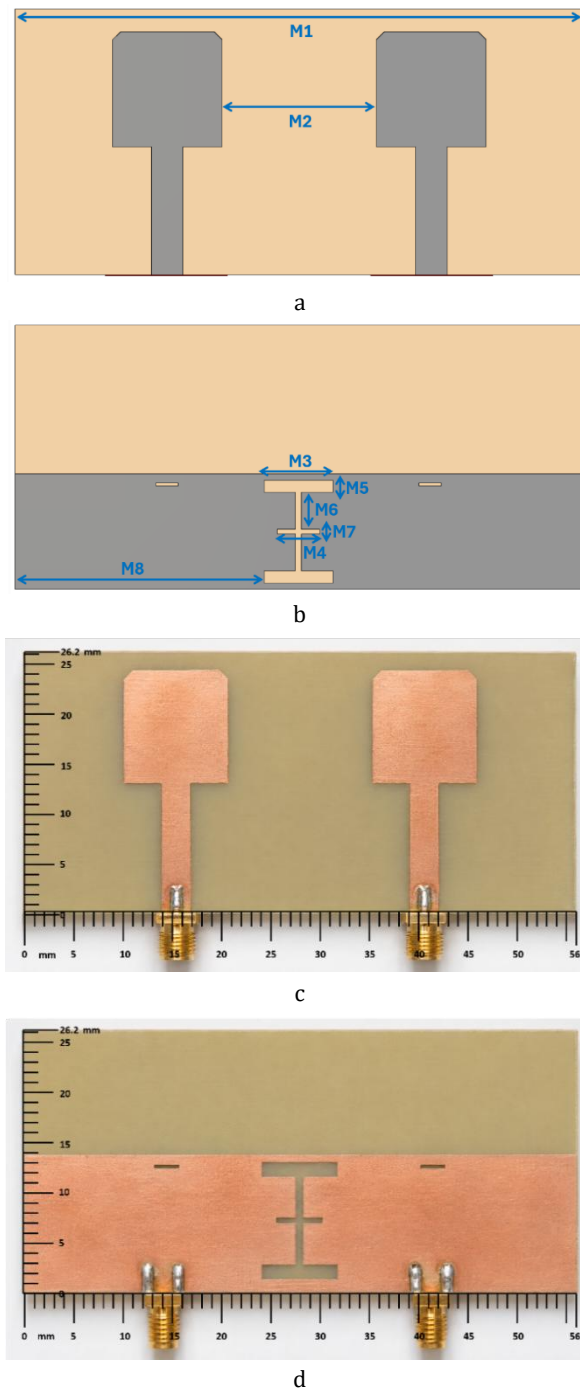
Figure 2. Geometry and fabricated prototype of the proposed MIMO antenna: (a) top view with design parameters, (b) bottom view with isolation design parameters, (c) fabricated prototype top view, and (d) fabricated prototype bottom view.
