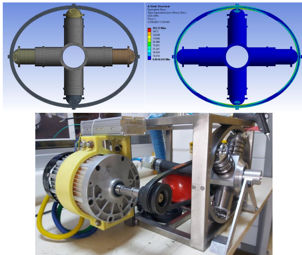
Figure 6. The manufactured prototype of the compressor.
