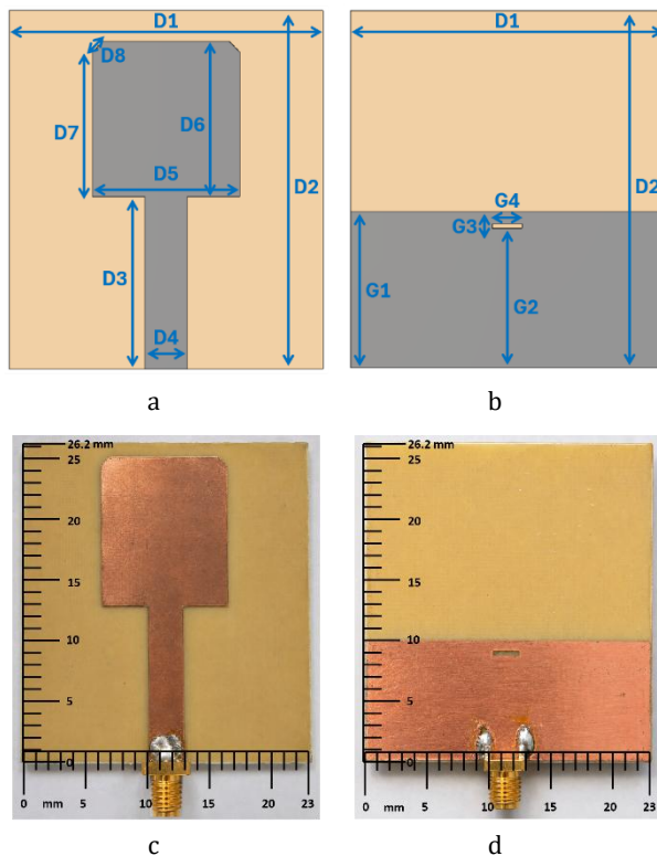
Figure 1. Geometry and fabricated prototype of the proposed antenna: (a) top view with radiator-side design parameters, (b) bottom view with partial-ground and defected-ground-slot parameters, (c) fabricated prototype top view, and (d) fabricated prototype bottom view.
