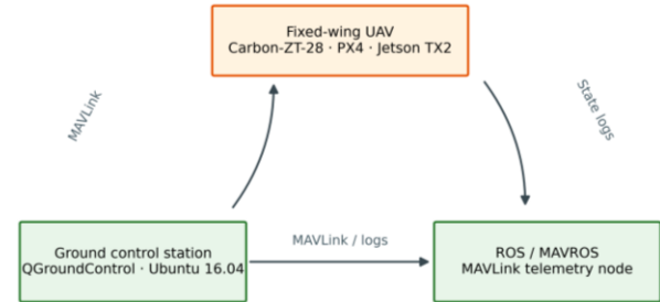
Figure 2. UAV-ground station telemetry architecture in the ALFA experimental setup (Keipour et al., 2019; Keipour et al., 2021).
