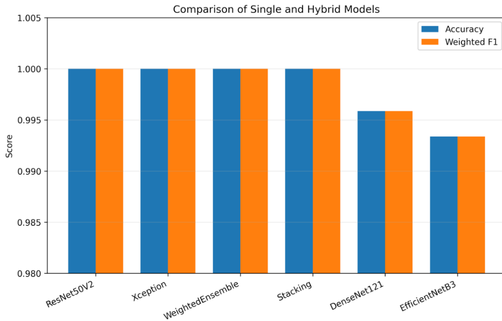
Figure 5. Comparative performance plot across single and hybrid models.
