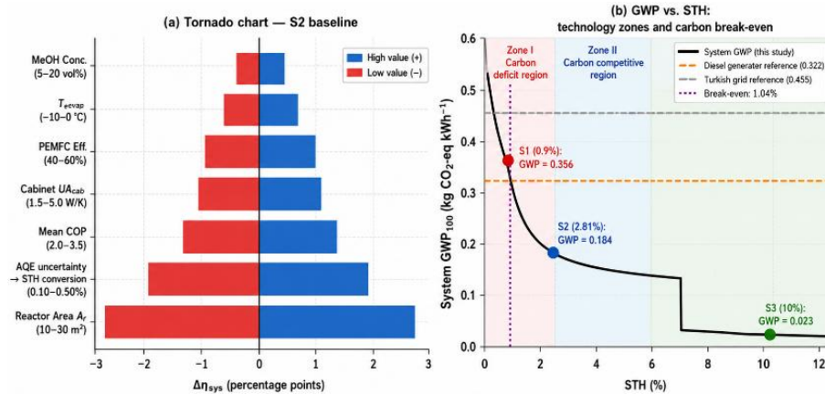
Figure 9. Sensitivity and carbon break-even analysis: (a) tornado chart showing sensitivity of \eta_{sys} to key design parameters; (b) system GWP 100 vs. STH with technology zones and the carbon break-even threshold (STH \approx 1.04%).
