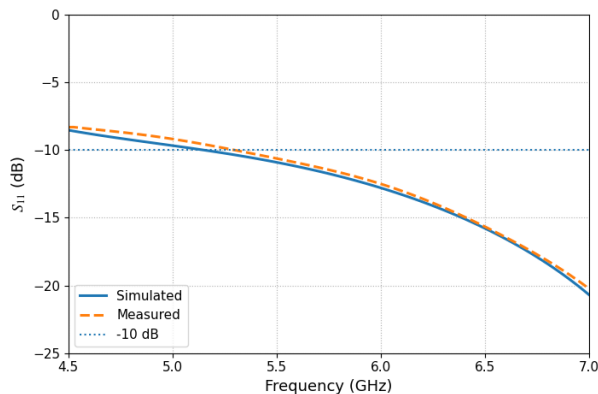
Figure 3. Simulated and measured reflection coefficient responses of the proposed single antenna.
