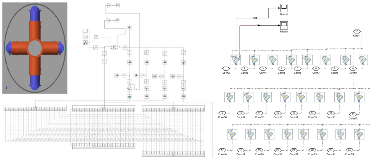
Figure 3. MATLAB/Simulink dynamics model of the compressor.
