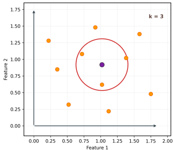
Figure 6. k-distance neighbourhood illustration in local outlier factor (Breunig et al., 2000).
