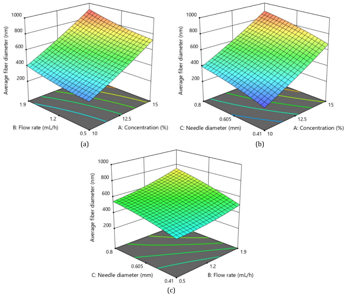
Figure 3. 3D response surface plots showing the combined effects of process parameters on r-PET AFD: (a) concentration–flow rate (AB), (b) concentration–needle diameter (AC), (c) flow rate–needle diameter (BC).
