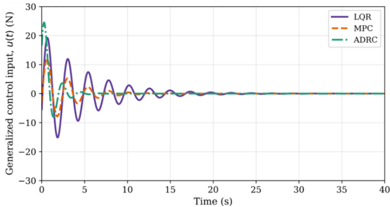
Figure 10. Generalized control input responses under Scenario 3.
