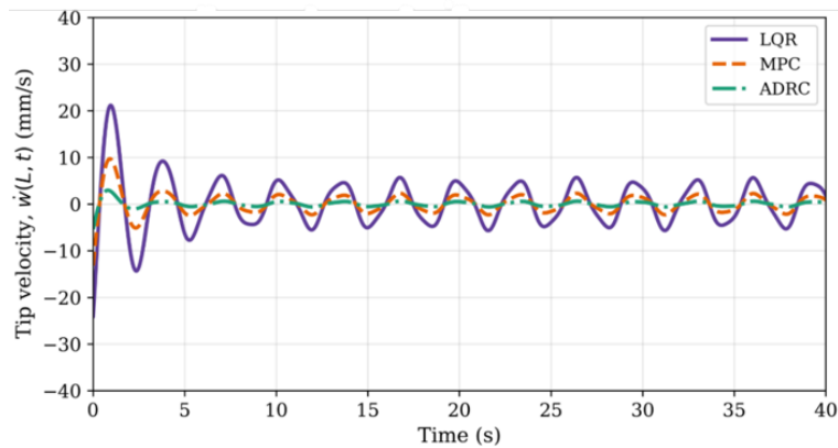
Figure 8. Tip velocity responses under Scenario 2.
