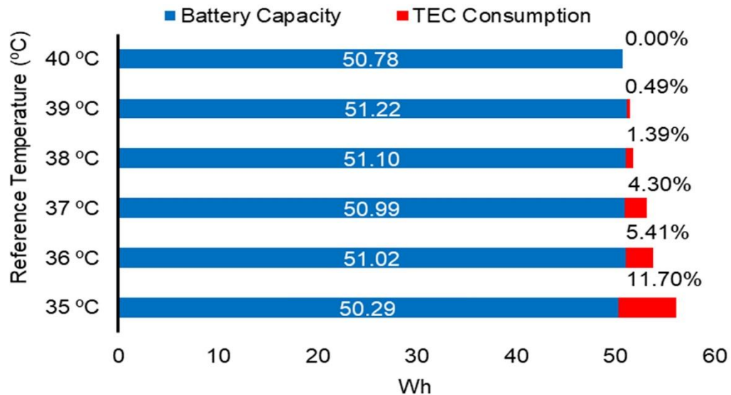
Figure 6. Comparison of battery energy capacity and TEC energy consumption, together with the corresponding energy-consumption ratios.
