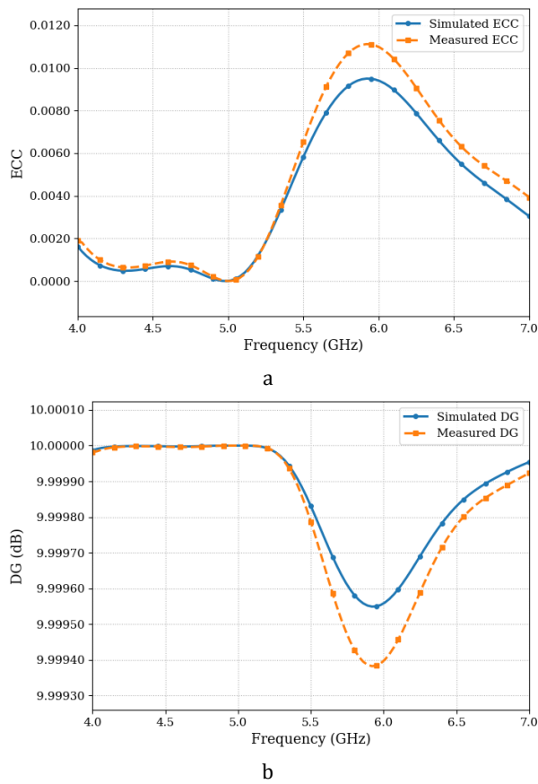
Figure 7. S-parameter-based diversity performance of the proposed two-port MIMO antenna calculated using the complete complex two-port data: (a) ECC and (b) DG.
