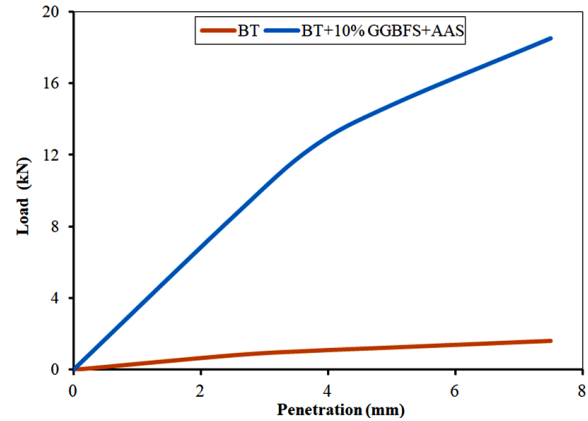
Figure 8. Load-displacement curves of untreated and 10% GGBFS+AAS stabilized specimens.
