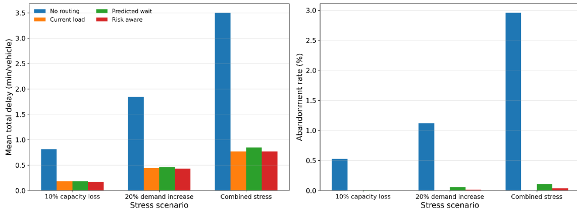
Figure 2. Simulation outcomes under the three stress scenarios with full recommendation acceptance. (a) reports mean total delay, including queueing time and the station-switching penalty. (b) reports queue-abandonment rates. All dynamic routing policies substantially reduced delay and nearly eliminated abandonment relative to no routing.
