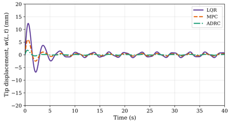
Figure 6. Tip displacement responses under Scenario 2.
