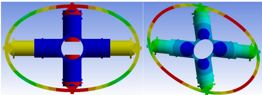
Figure 5. First and second mode shapes of the compressor mechanism.
