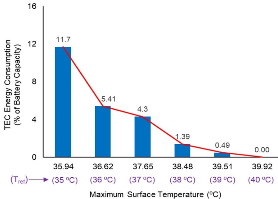
Figure 7. Variation of auxiliary energy consumption with maximum battery surface temperature.
