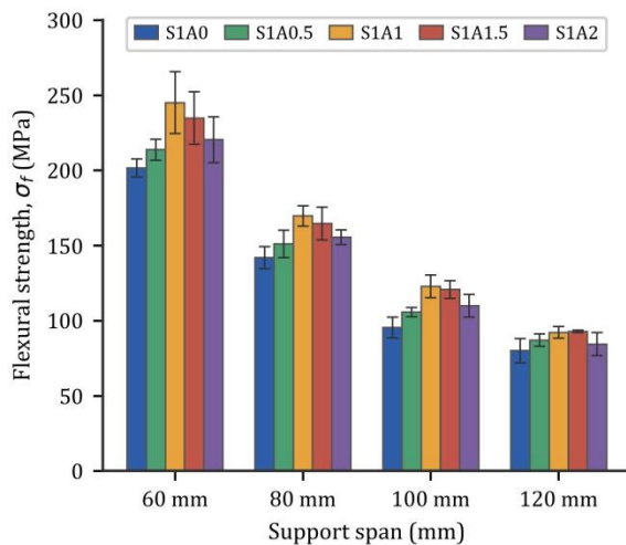
Figure 3. Flexural strength by support span.
