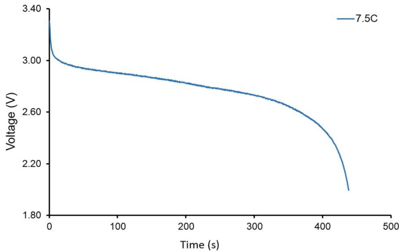
Figure 3. Representative battery voltage profile during a 7.5C discharge test.
