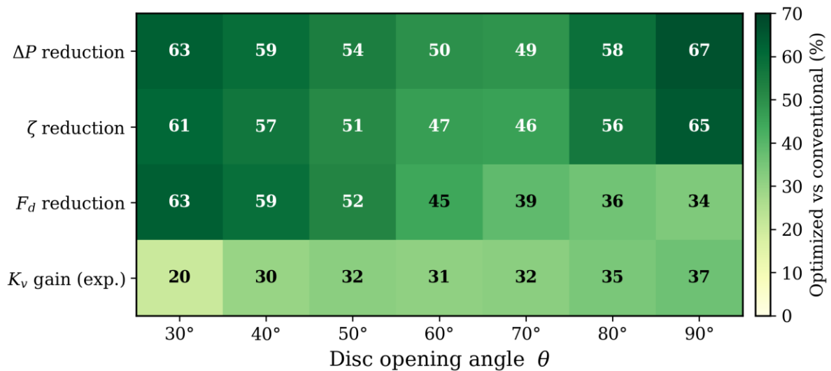
Figure 9. Performance map of the optimized versus the conventional design across four basic metrics (pressure-loss reduction, loss-coefficient reduction, hydrodynamic-force reduction and experimental Kv increase) and seven opening angles. All cells are positive (green). That is, the optimized disc improves every metric at every angle.
