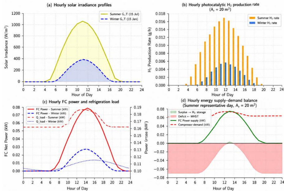
Figure 7. Seasonal performance comparison on representative days (S2 baseline): (a) hourly solar irradiance; (b) hourly H_2 production rate; (c) FC power and refrigeration load; (d) hourly energy supply-demand balance with surplus/deficit areas.
