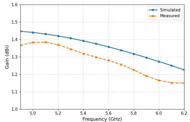
Figure 4. Simulated and measured gain responses of the proposed single antenna.
