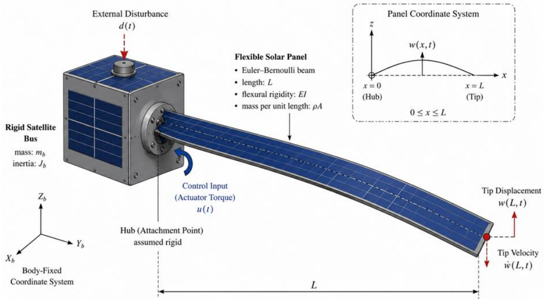
Figure 1. Physical Configuration of the rigid-flexible satellite system.
