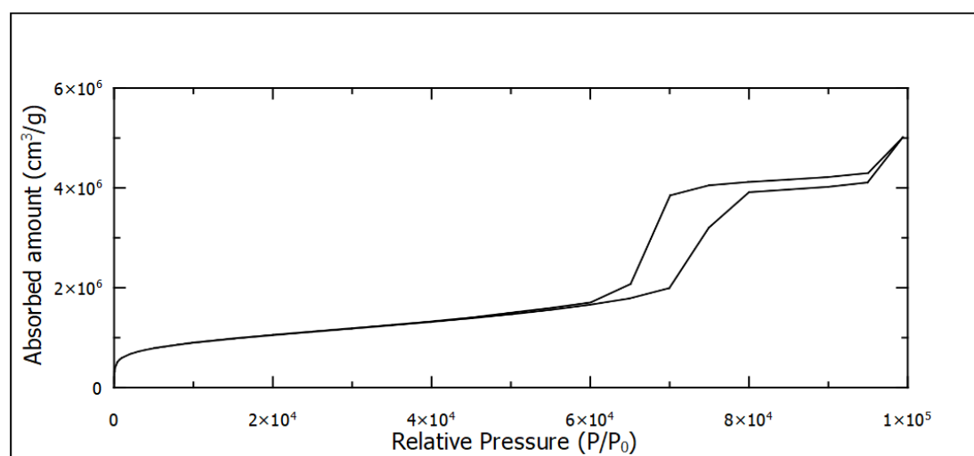
Figure 5. N 2 adsorption/desorption isotherm of SBA-15.
