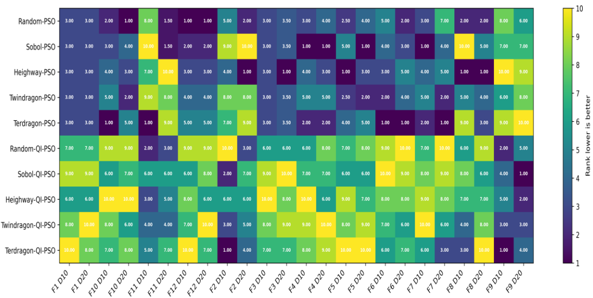
Figure 6. CEC 2022 function dimension rank heatmap.
