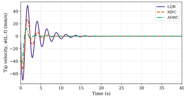
Figure 5. Tip velocity responses under Scenario 1
