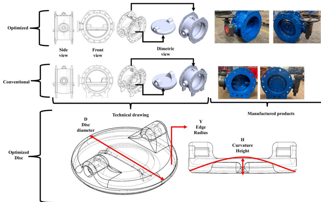
Figure 2. Conventional (bottom) and optimized (top) valve designs. On the left are the side and front technical drawings and the exploded three-dimensional CAD models of the body and disc in dimetric view. On the right are the manufactured products with their geared actuators. At the bottom, the optimized disc technical drawing is shown, defining the patented design rule parameters, namely the disc diameter D, the edge oval radius Y and the curvature height H.
