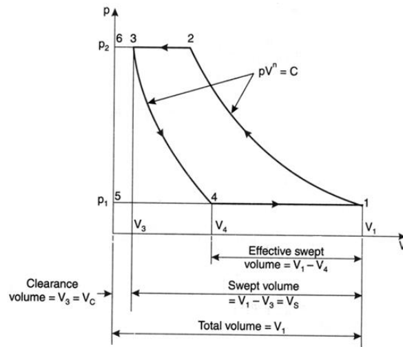
Figure 2. The thermodynamic cycle of the compressor.
