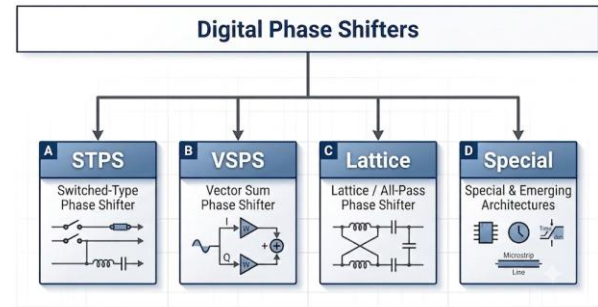
Figure 1. Proposed taxonomy of digital phase-shifter architectures based on the primary phase-generation mechanism.
