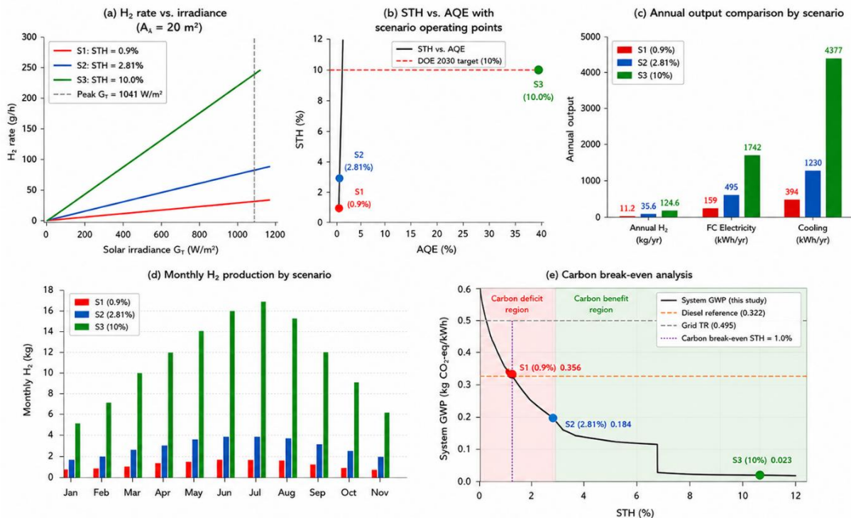
Figure 2. Photocatalytic H 2 production characteristics and three-scenario framework ( A_r=20 \text{ m}^2 ): (a) H 2 production rate vs. solar irradiance; (b) STH vs. AQE with scenario operating points; (c) annual output comparison; (d) monthly H 2 production; (e) carbon break-even analysis (STH threshold \approx 1.04\% ).
