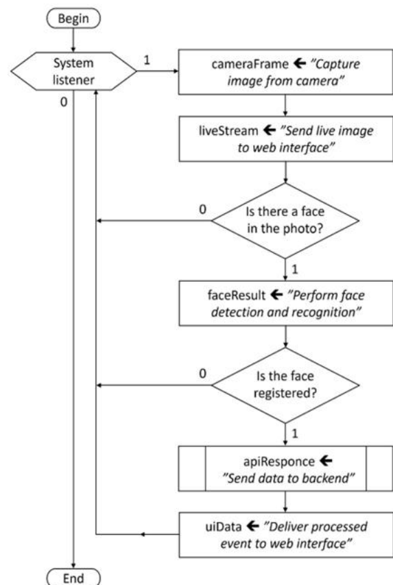
Figure 3. Flowchart of the facial recognition system.
