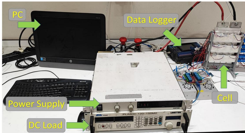
Figure 2. Experimental setup.
