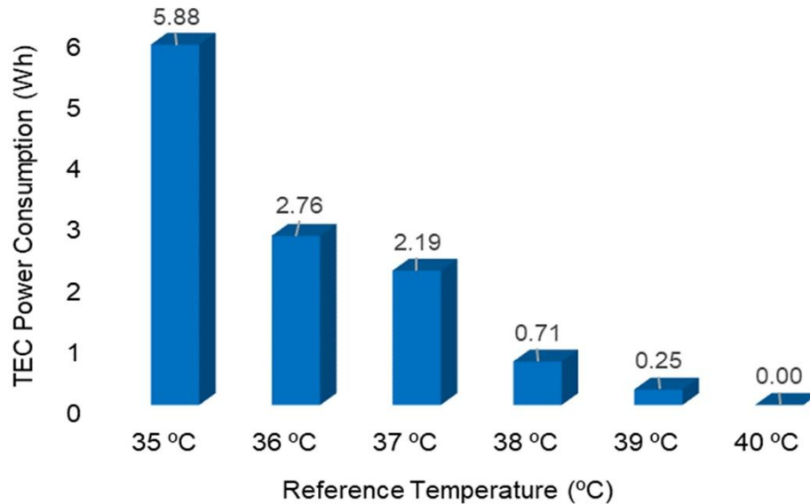
Figure 5. Effect of reference temperature on the total energy consumption of the TEC modules.
