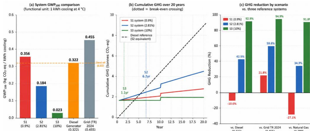
Figure 10. Life cycle assessment results: (a) GWP 100 by scenario vs. reference systems; (b) cumulative GHG trajectories over 20-year lifetime; (c) GHG reduction by scenario vs. three reference systems.
