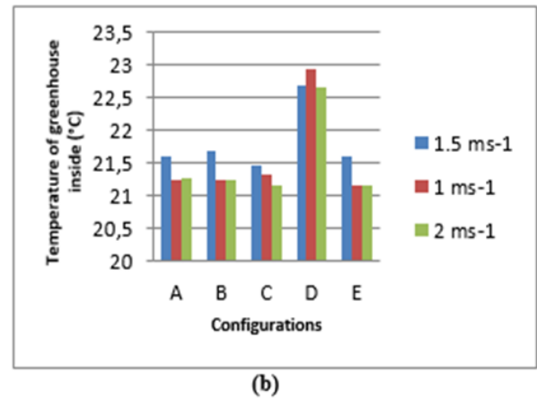
Figure 3. Temperature distribution of configurations at different wind speed on May (a) and June (b)
