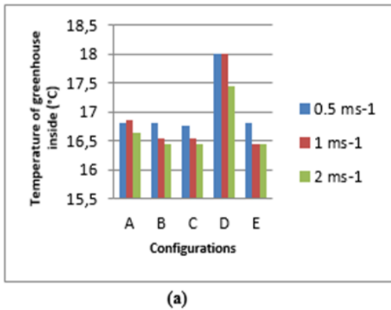
Figure 3. Temperature distribution of configurations at different wind speed on May (a) and June (b)
