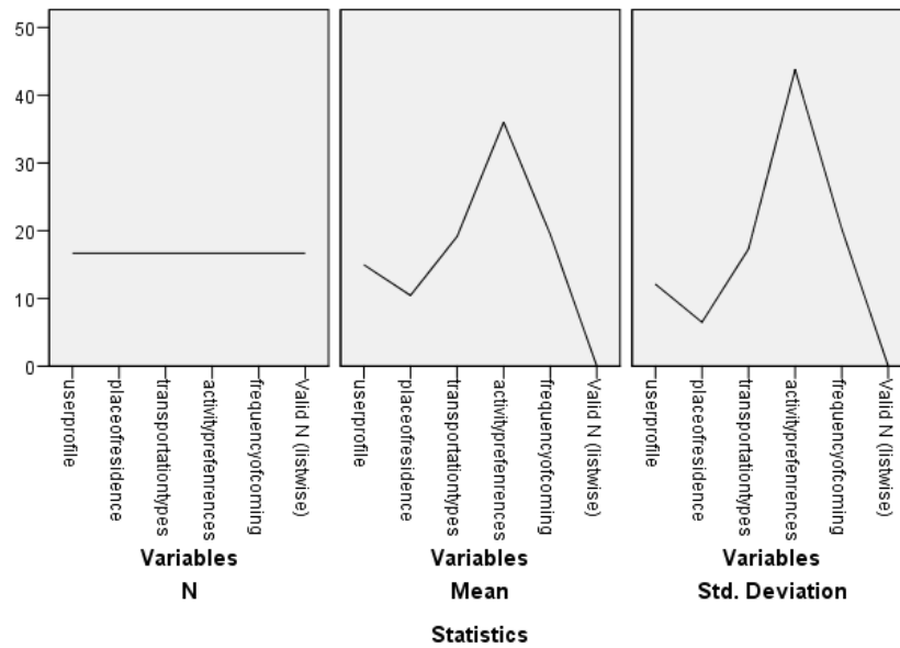
Figure 7; Descriptive statistic
