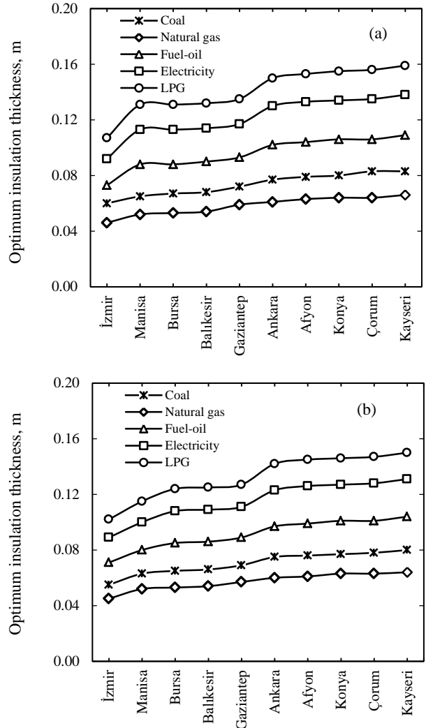
3. Optimum insulation thickness for (a) RW and (b) GW in selected cities
