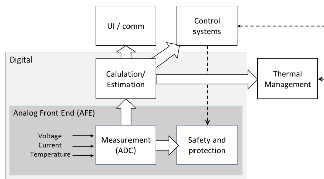
Figure 7 Digital BMS functional schematic
