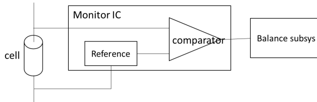
Figure 2 Analog BMS example circuit (Andrea, 2010)
