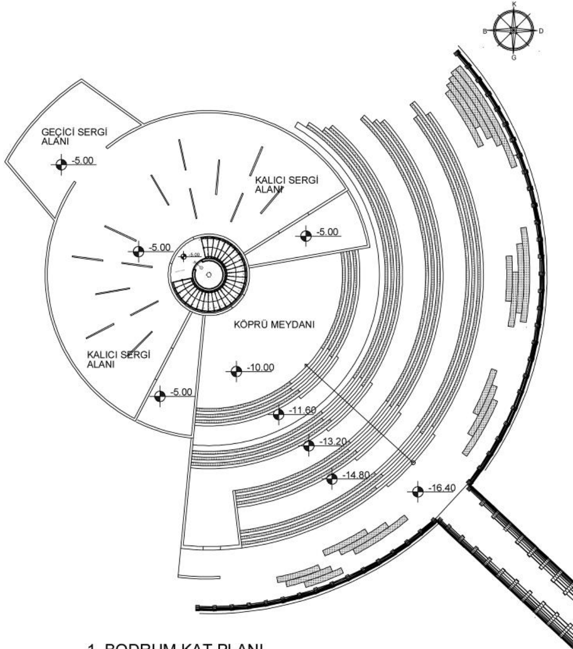
-1. BODRUM KAT PLANI
