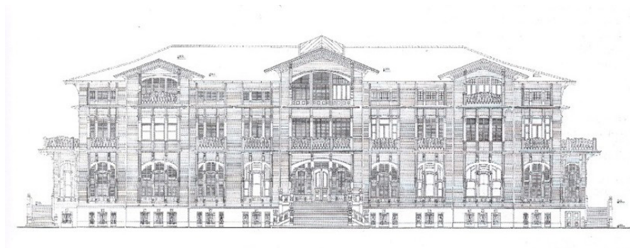
Figure 4. Ahmed Ratib Paşa Mansion Main façade drawing by Ali Hacıhaliloğlu (Yavuz, Y. 2009a: 89-90)
