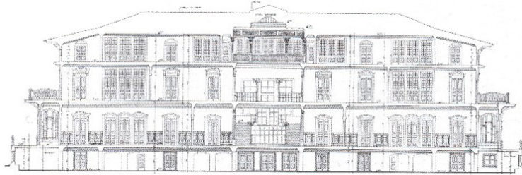
Figure 5. Ahmed Ratib Paşa Mansion Section drawing by Ali Hacıhaliloğlu (Yavuz, Y. 2009a: 89-90)
