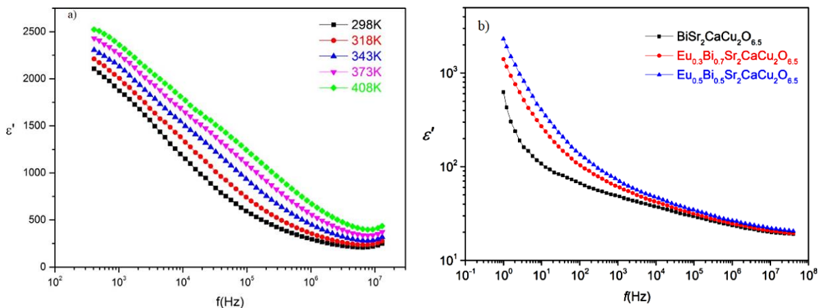
Figure 3. a) Frequency dependence of the real components of the complex dielectric functions at different temperatures for Eu-1223 material [3]. b) for the (Eu x Bi 1-x )-212 samples ( x=0, 0.3, 0.5 ) at room temperature [2].
