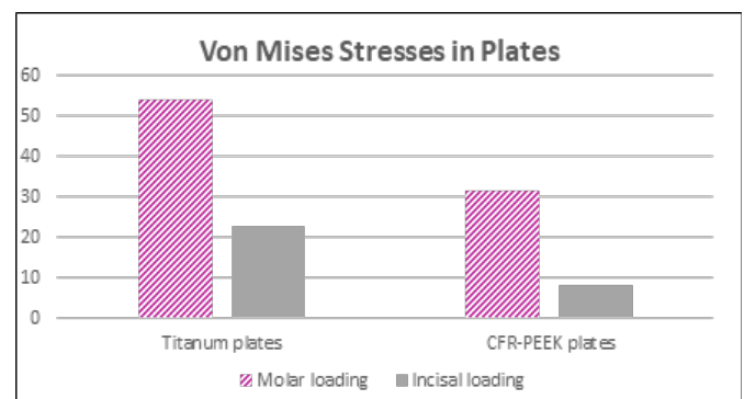
Figure 2. Von Mises stresses in plates
