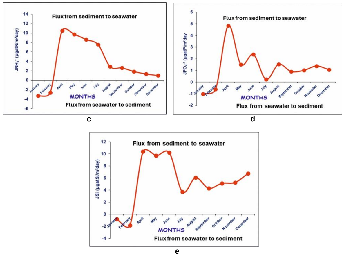
Figure 8. The monthly variation of NO 3 - (a), NO 2 - (b), NH 4 + (c), PO 4 3- (d) and Si (e) obtained from core incubations at Homa Lagoon surface sediment
